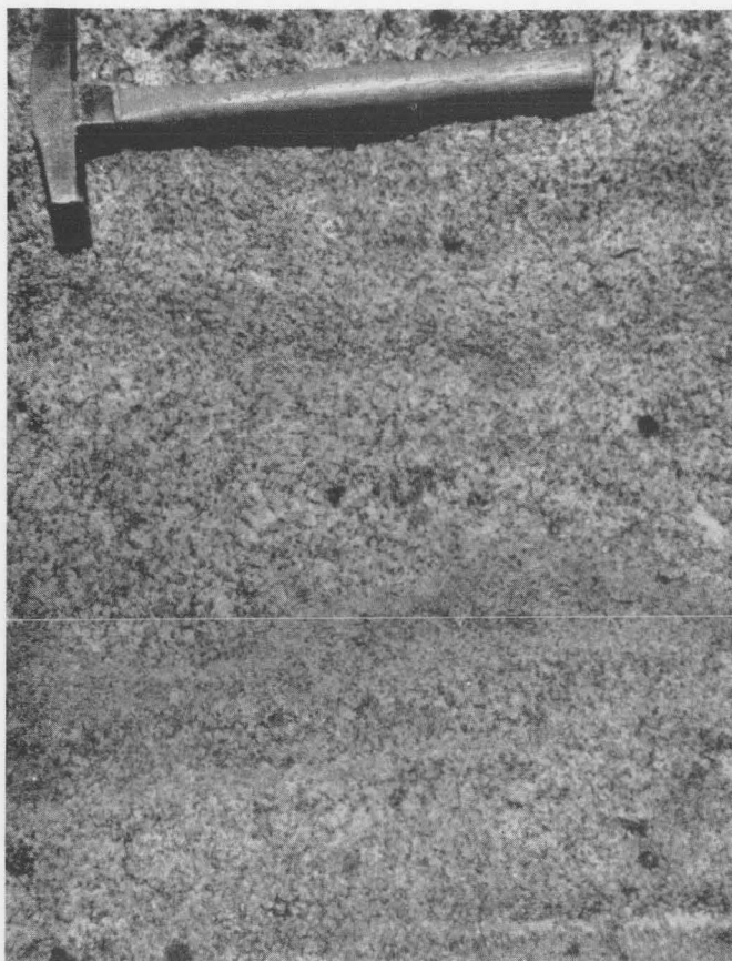
Plate IV, Fig. A. Fine textural layering in fine-grained granite.
