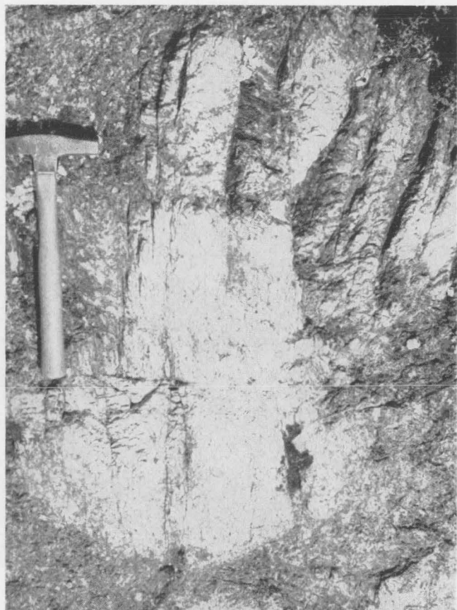
Plate IV, Fig. B. Large porphyritic graphic granite crystal in a matrix of coarse-grained granite.
