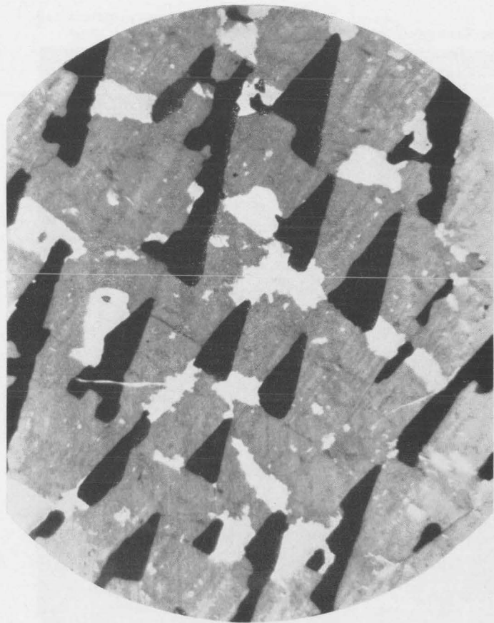
Plate V, Fig. B. Graphic granite crystal showing relations of microcline, quartz, and plagioclase. Quartz is black, microcline is gray, and plagioclase is white. Crossed nicols; X 26.
