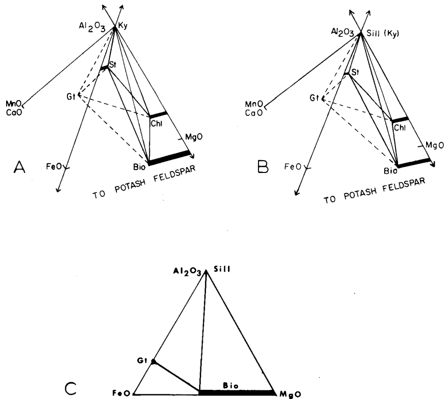
Fig. 5. Diagrams A and B are modified Thompson projections for pelitic schist in the Newtown quadrangle. Mineral regions in the face Al_2O_3 , FeO, MgO are determined by lines projected through muscovite in the compositional tetrahedron K_2O , Al_2O_3 , FeO, MgO. Minerals shown are coexisting with quartz, plagioclase, muscovite, and magnetite. Chlorite in both projections is retrograde, which explains the crossing tie lines kyanite-biotite and staurolite-chlorite. Phase regions for staurolite, biotite, and chlorite are hypothetical. Numerous theoretical tie lines exist between all minerals, providing they do not cross. These are not shown because the appropriate bulk compositions were not observed. Diagram A shows assemblages east of the first sillimanite isograd and diagram B contains assemblages to the west. The schematic phase regions are different in B because sillimanite develops from both muscovite and biotite, thus contributing K_2O , MgO, and FeO to coexisting minerals. Data for diagram A is based in part on sample 731 of table 1. Diagram C is projected through potash feldspar in the same compositional tetrahedron as diagrams A and B for samples west of the second sillimanite isograd. Minerals are kyanite (Ky), staurolite (St), garnet (Gt), chlorite (Chl), biotite (Bio), sillimanite (Sill).
