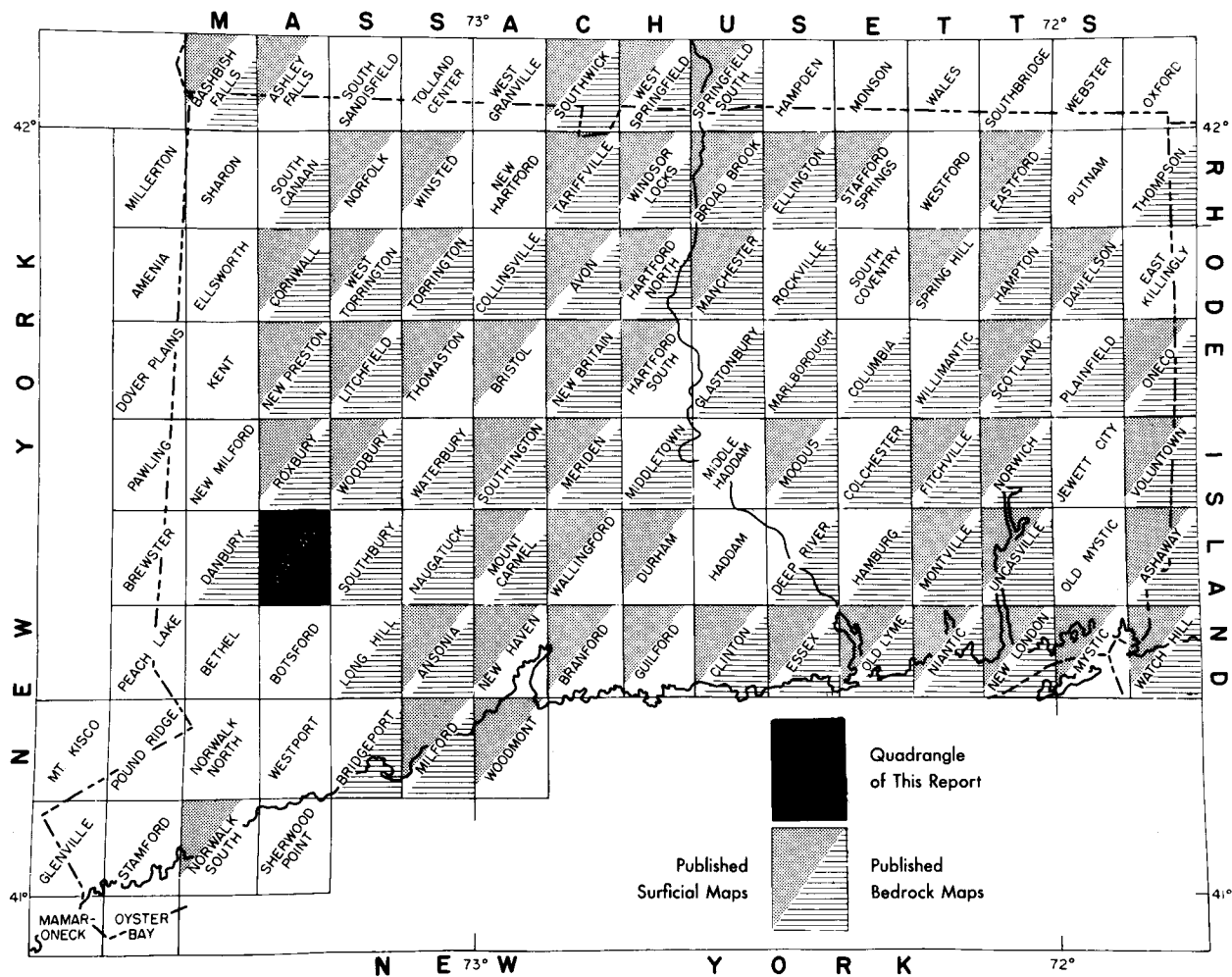
Fig. 1. Index map of Connecticut, showing the location of the Newtown quadrangle and of other published quadrangle maps.
