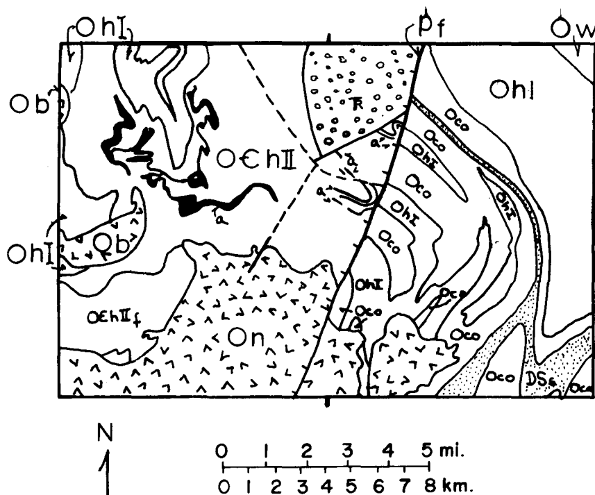
Fig. 11. Geologic map of the Newtown and Southbury quadrangles, showing distribution of Hartland II (OChII), the amphibolite in Hartland II (a), the feldspathic schist in Hartland II (OChII f), the Waterbury Formation (Ow), Hartland I (OhI), the Collinsville Formation (Oco), the Straits Schist (DSs), the Brookfield Gneiss (Ob), the Newtown Gneiss (On), and the rocks of Triassic age (R). The faults correspond to those on plate 1. The Pomperaug fault is marked pf .
