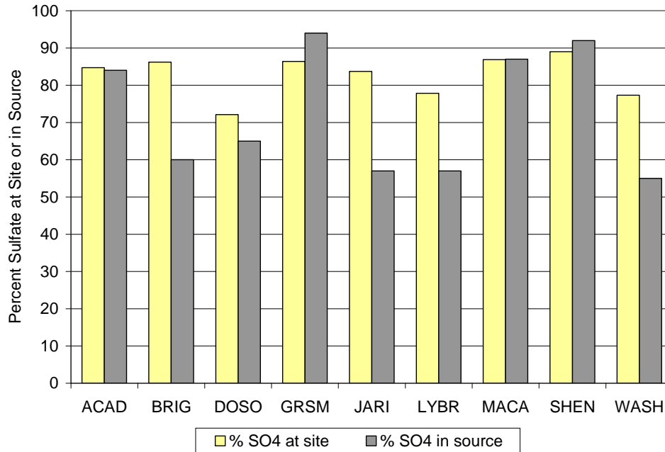
Figure 5-5. Sulfate characteristics of “secondary sulfate” (coal) sources identified at eastern sites
