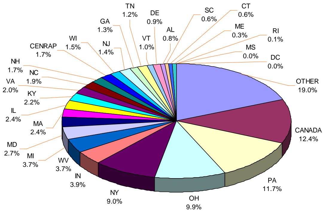
Figure 6-6. 2002 Eastern states' contribution to annual PM sulfate in Lye Brook, VT
