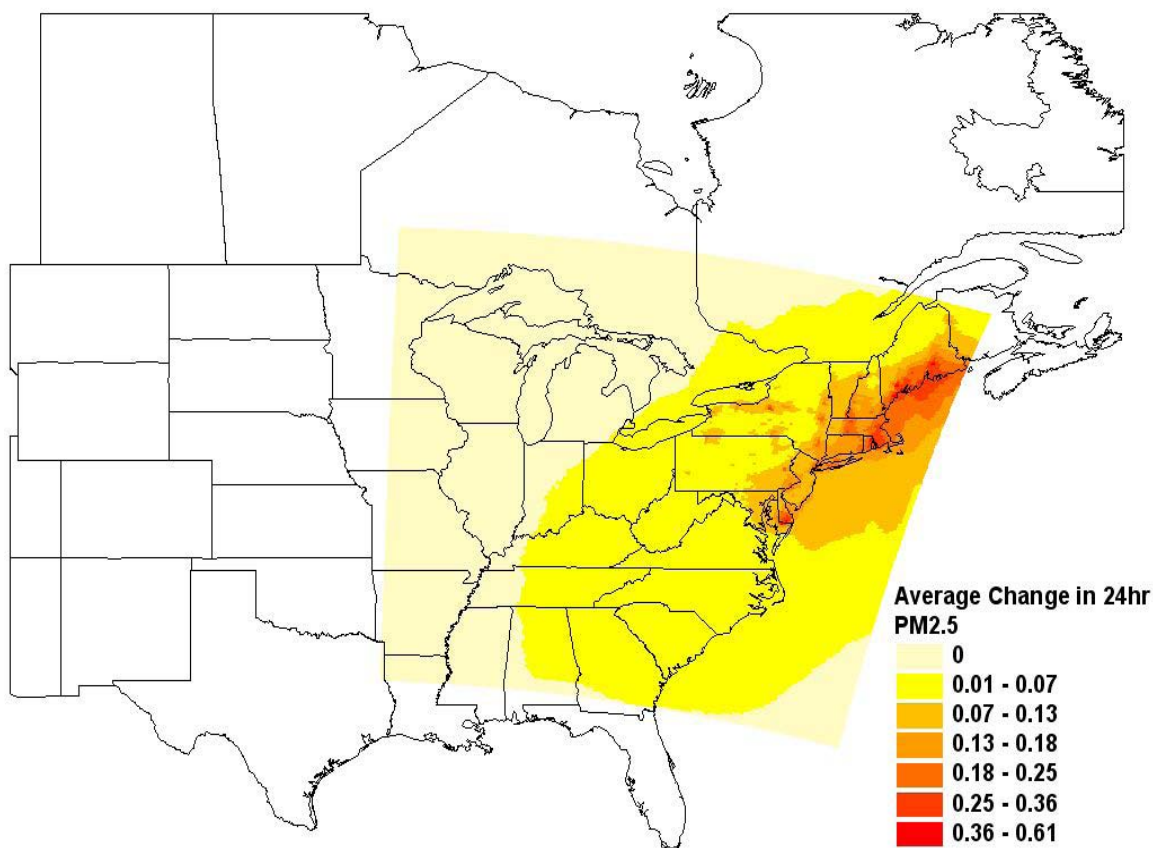
Figure 10.1: Average Change in 24-hr PM 2.5 Due to Low-Sulfur Fuel Strategy (Phases I and 2 Combined) Relative to OTB/OTW (values in µg/m 3 )
