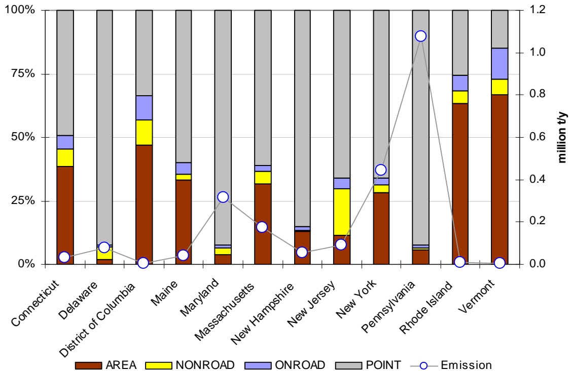
Figure 8.12: 2002 Sulfur Dioxide (SO 2 ) Emissions, by State Bar Graph = Percentage Fractions of Four Source Categories Line Graph = Total Annual Emissions (10 6 tpy)
