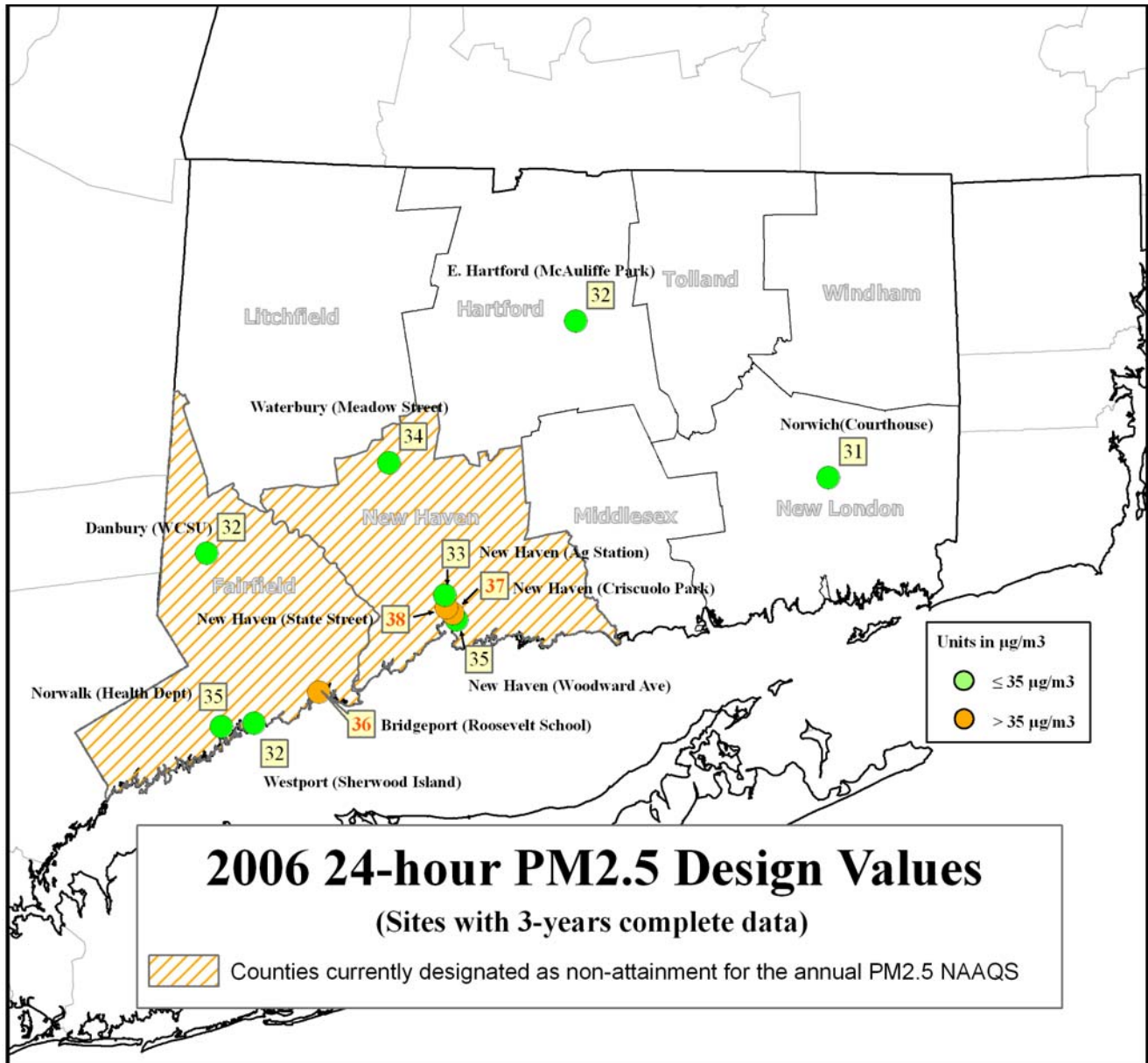
Figure 1. Map of PM 2.5 Monitors in Connecticut with valid 2006 Design Values
