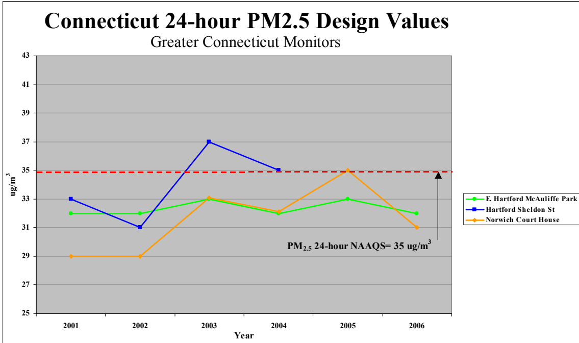
Figure 2. Graph of 24-hour Design Values for Greater Connecticut, 2001-2006
