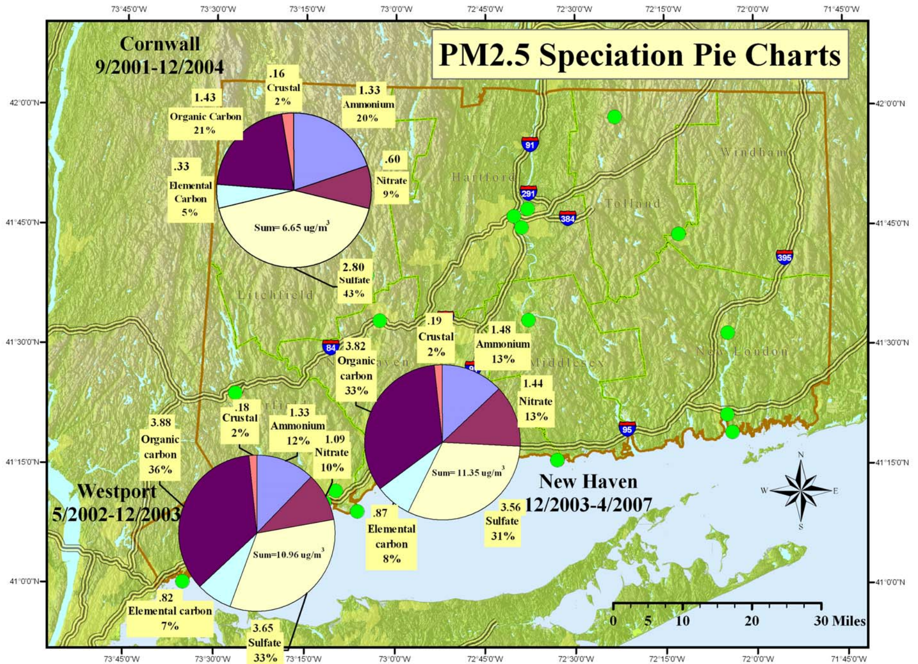
Figure 11. PM 2.5 Speciation Pie Charts
