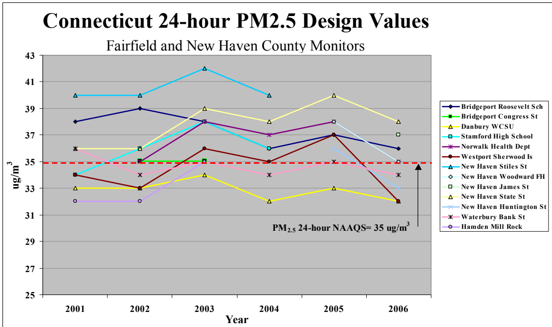
Figure 3. Graph of 24-hour Design Values for Fairfield and New Haven Counties, 2001-2006
