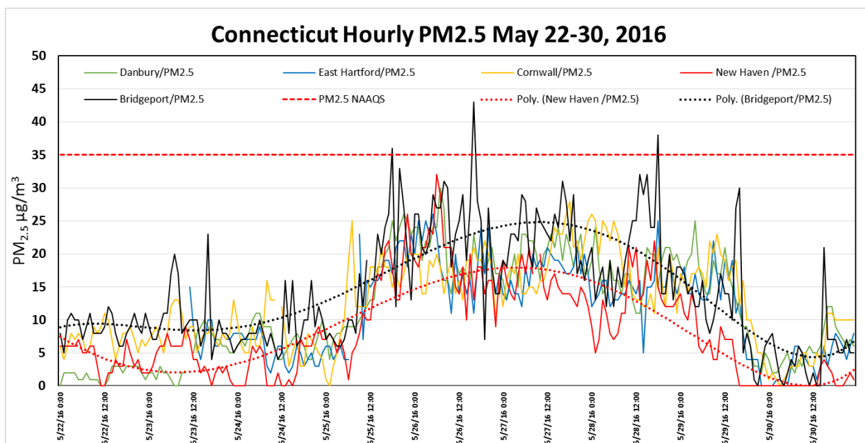
Figure 37. Hourly PM 2.5 Concentrations Recorded at Connecticut Monitors from May 22-30, 2016
