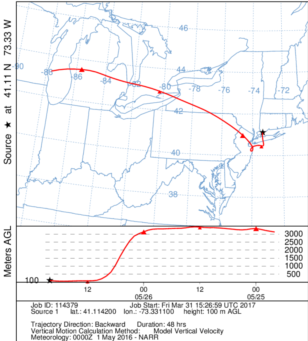
Figure 75. 100 meter Back Trajectory from Westport Connecticut ending at 4:00 pm LDT, May 26, 2016.
