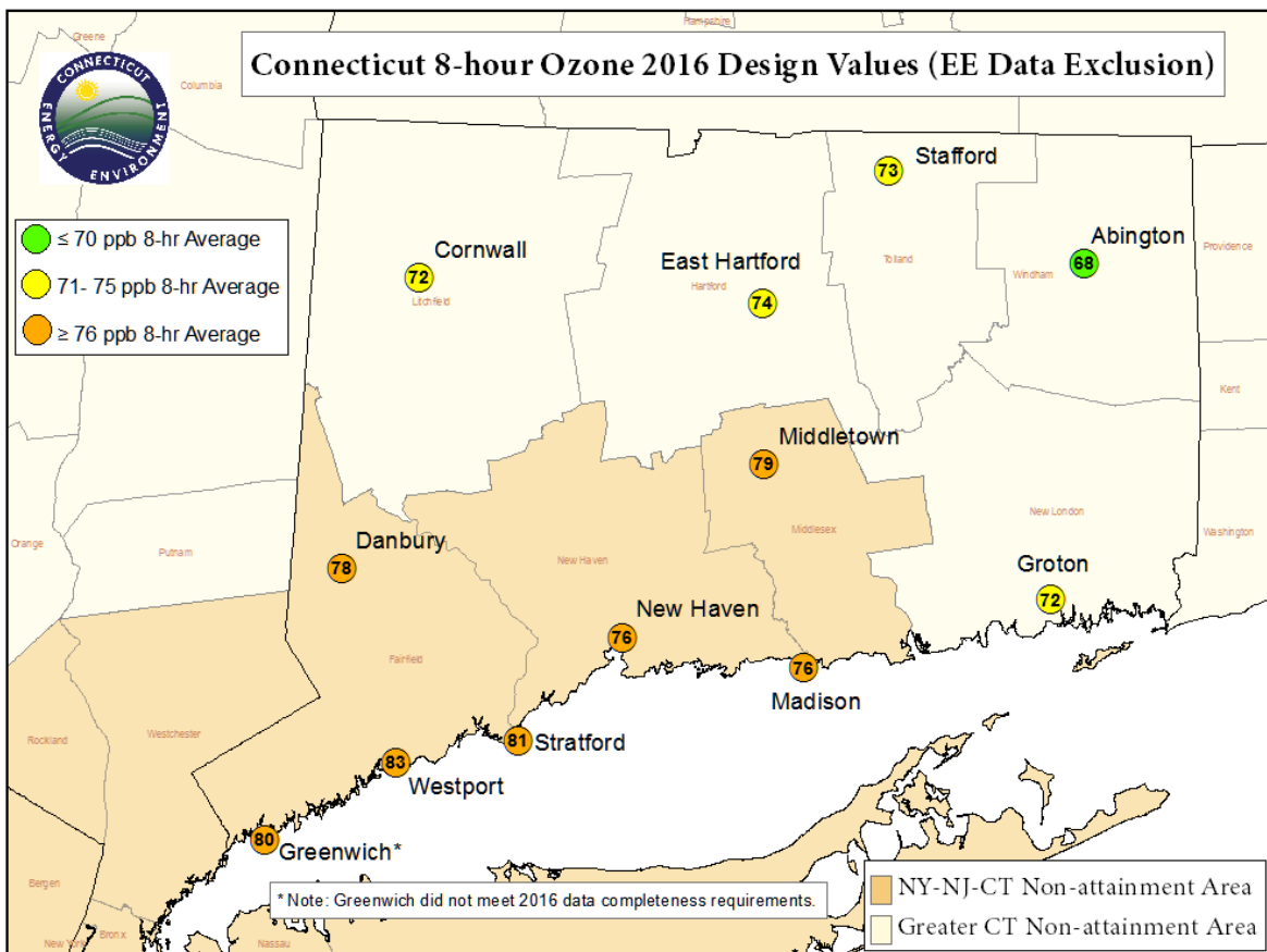
Figure 93. Map of 2016 Connecticut 8-hour Ozone design Values after Data Exclusion.
