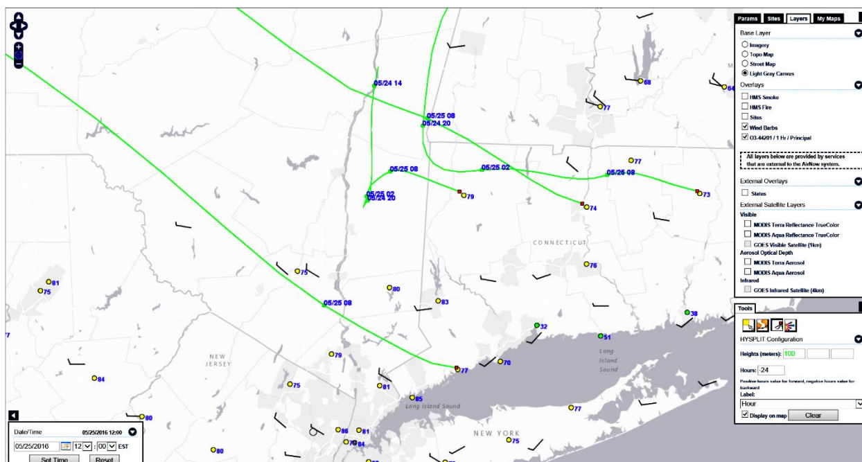
Figure 76. May 25th 24-hour Back Trajectories ending at 12:00 EST.
