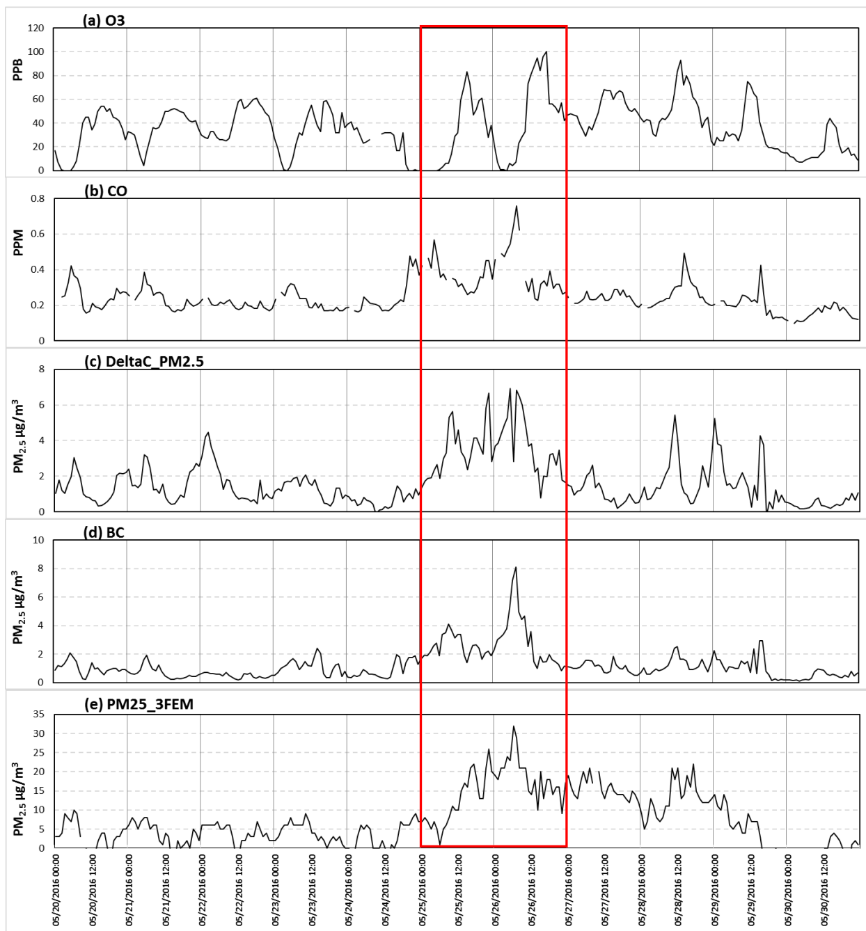
Figure 41. Monitored (a) Ozone, (b) Carbon Monoxide (CO) (c) DeltaC PM2.5 (d) Black Carbon (BC), and (e) PM2.5 at the New Haven CT Monitor
