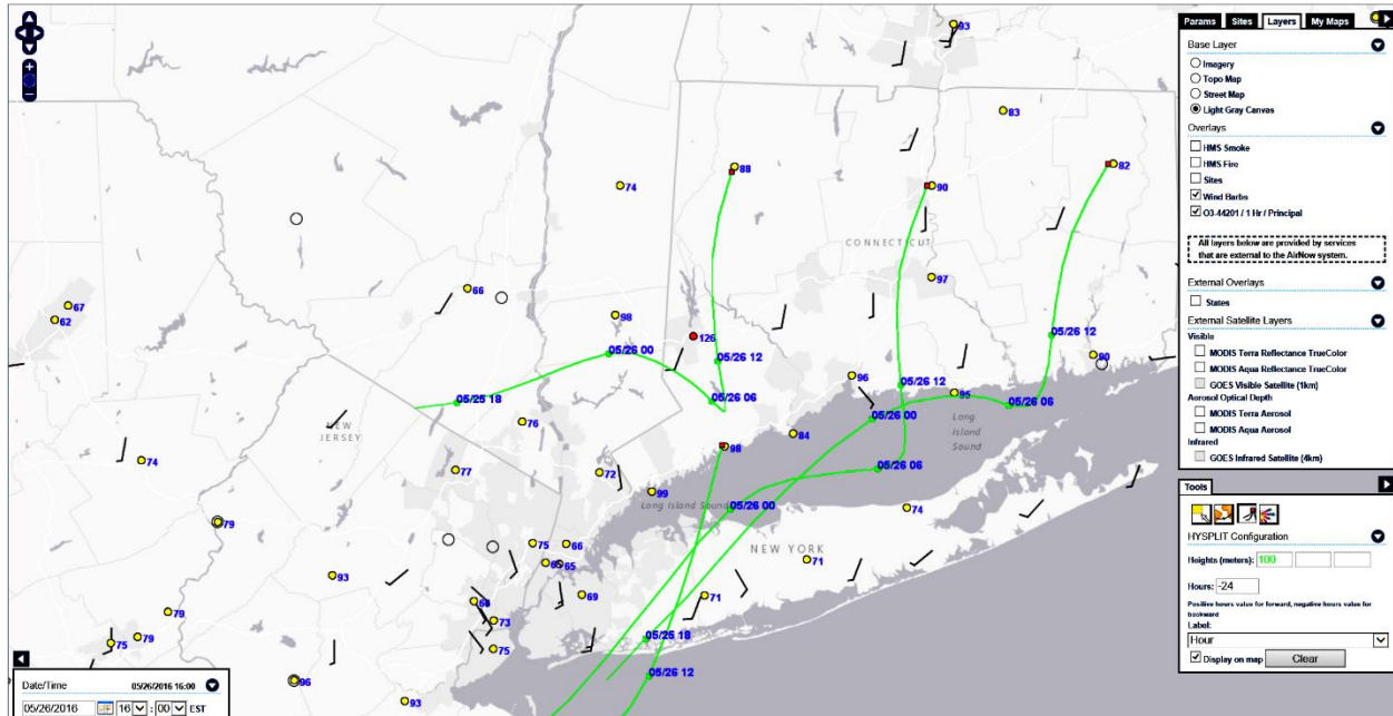
Figure 77. May 26th 24-hour Back Trajectories ending at 16:00 EST.
