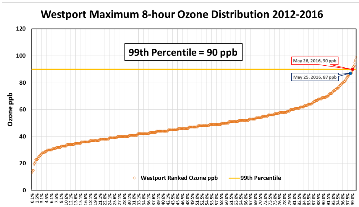
Figure 31. Ranked 8-hour Ozone Distribution for Westport CT 2012-2016
