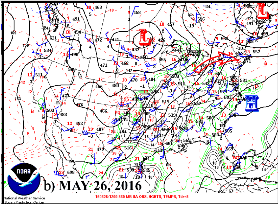
Figure 57. 850 mb Pressure Pattern with Winds for May 25-26 (a,b), 2016. High pressure center moves off the east coast causing the 850 mb transport winds to turn more westerly from Michigan.
