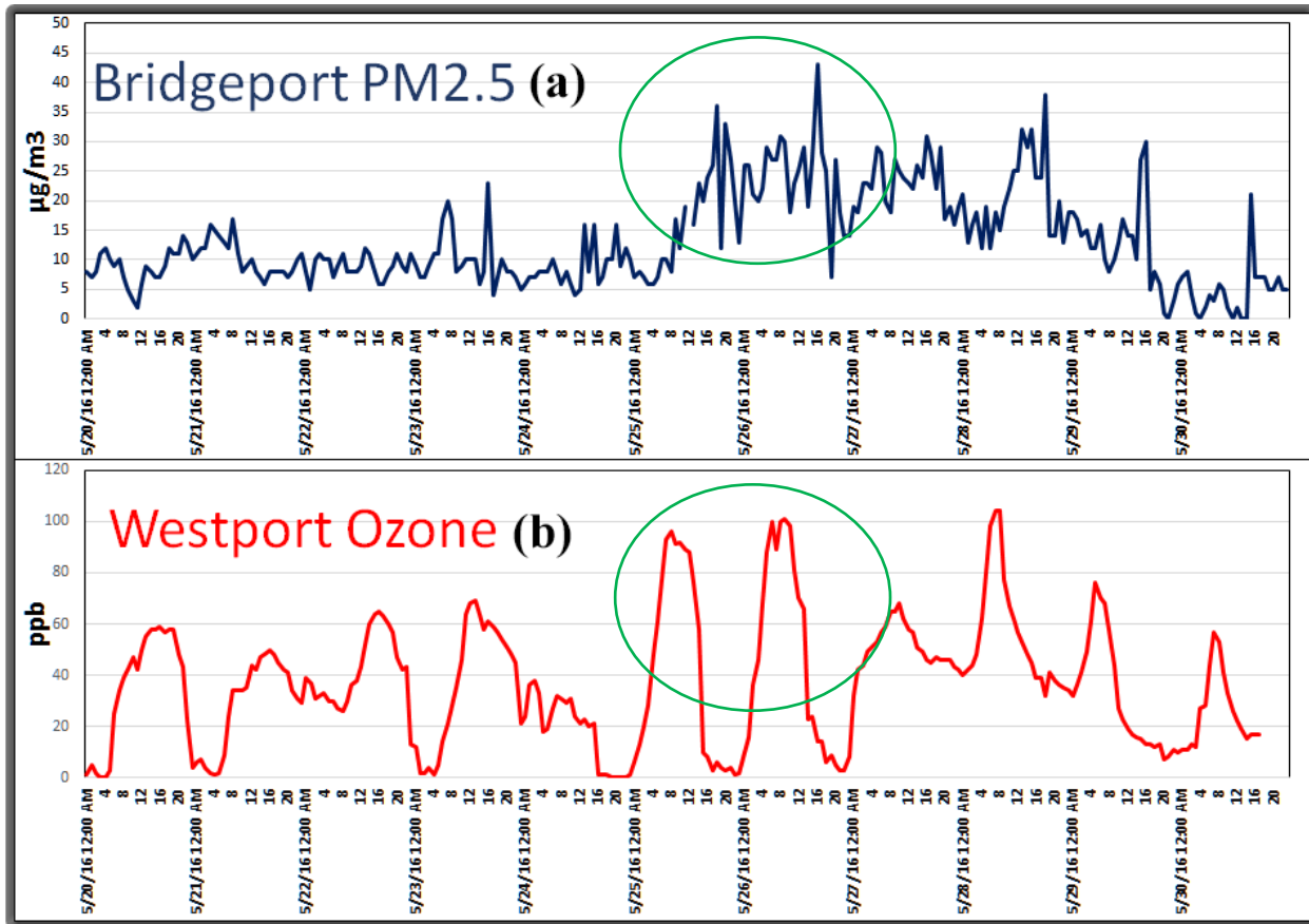
Figure 17. May 20-30, 2016 plots of (a) Bridgeport CT PM2.5 and (b) Westport Ozone Hourly Concentrations. The ozone peaks at Westport on May 25-26 coincide with the PM2.5 peaks at the Bridgeport monitor.
