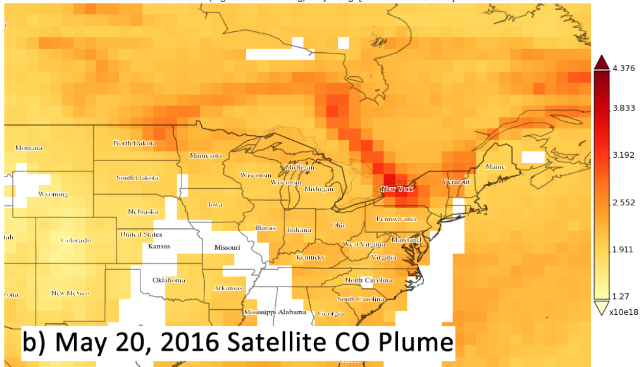
Figure 14. Satellite CO Plume from May 19 (a) and May 20 (b) , 2016. The plume meanders across southern Canada into the U.S. Midwest and across Connecticut.
