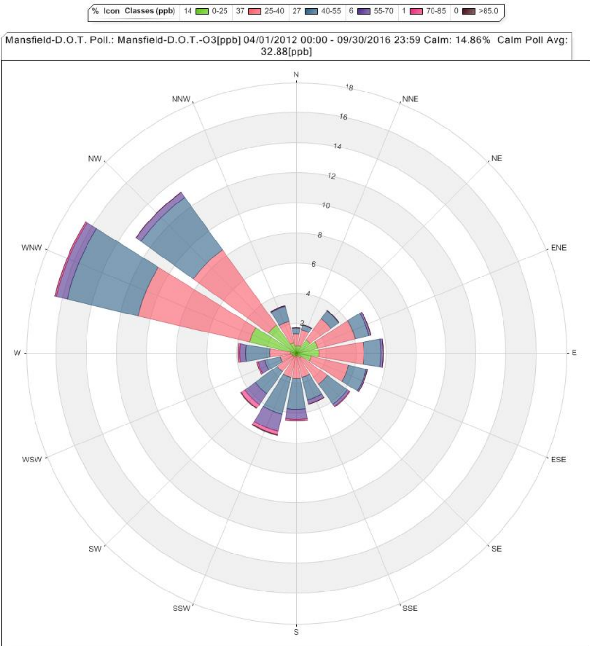
Figure 23. Ozone Wind Rose from Abington Connecticut.
