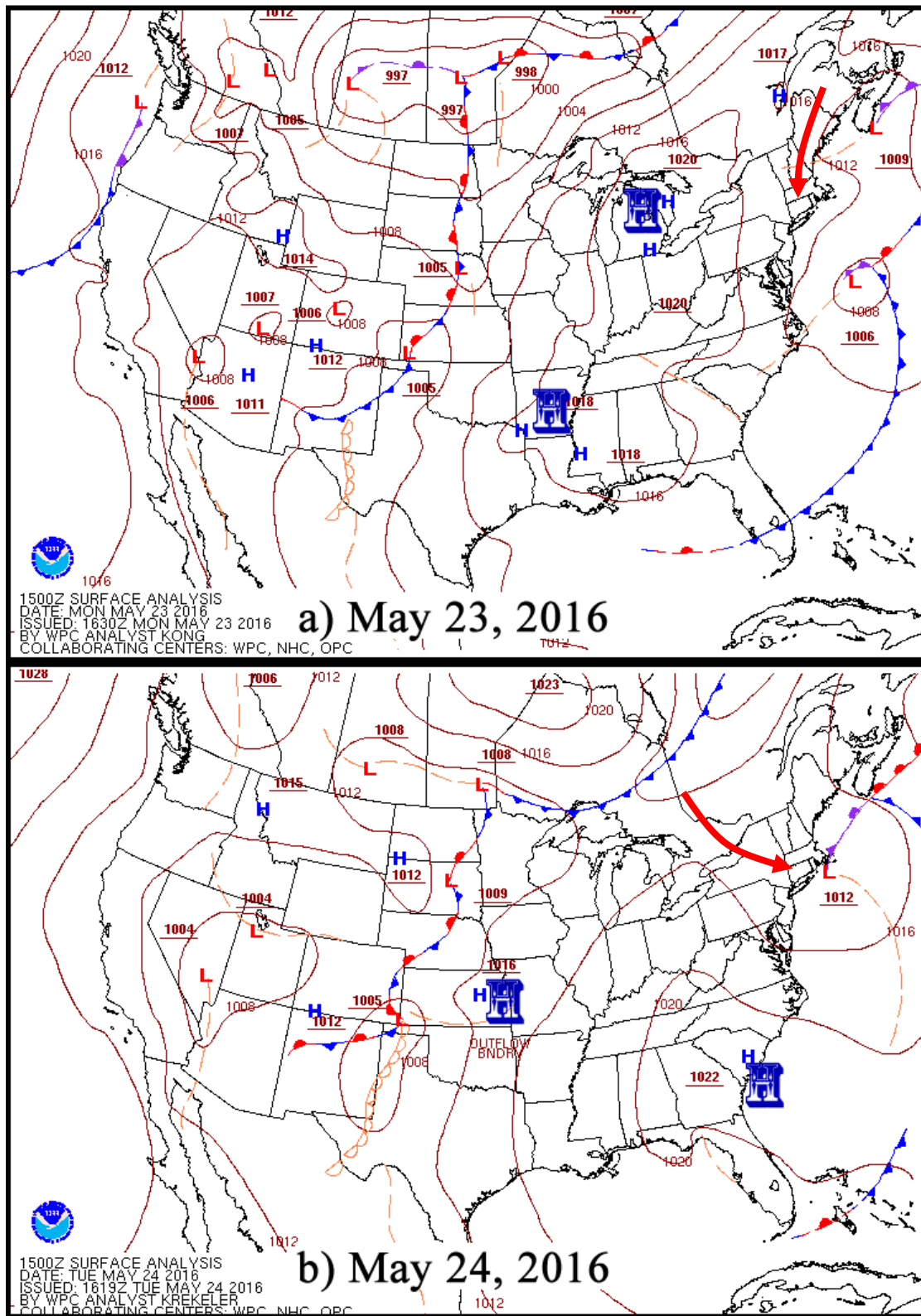
Figure 54. Surface Fronts for May 23-24 (a,b), 2016. Note the high pressure area over the Midwest on May 23-24th, creating subsidence and trapping the smoke plume pollutants over the Midwest.
