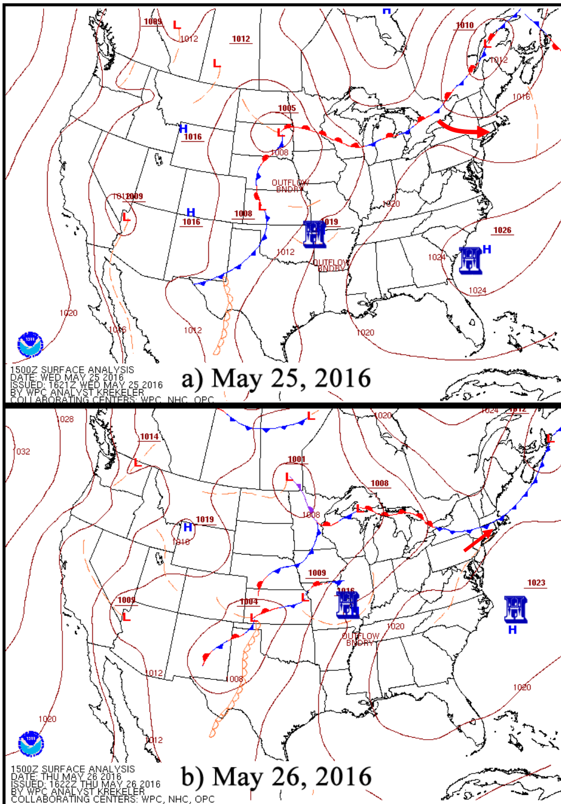
Figure 55. Surface Maps for May 25-26 (a,b), 2016. This shows northwest winds at the surface with approaching coldfront (a) turning the winds to the southwest(b) on May 26th.
