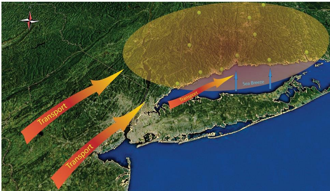
Figure 3. State-wide Ozone Exceedance Scenario
