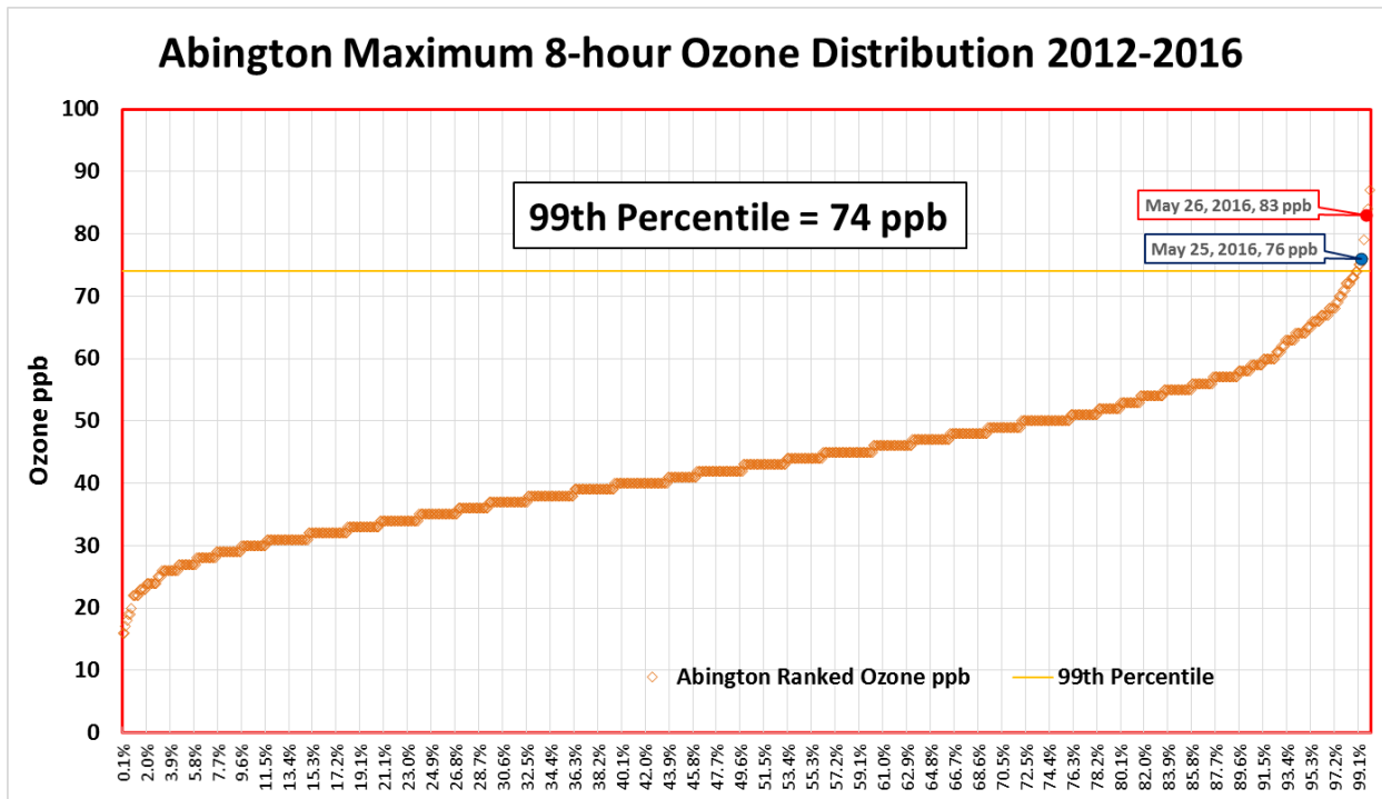
Figure 29. Ranked 8-hour Ozone Distribution for Abington CT 2012-2016
