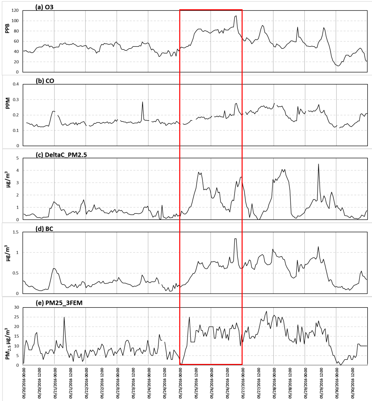
Figure 39. Monitored (a) Ozone, (b) Carbon Monoxide (CO) (c) DeltaC PM2.5 (d) Black Carbon (BC), and (e) PM2.5 at the Cornwall CT Monitor
