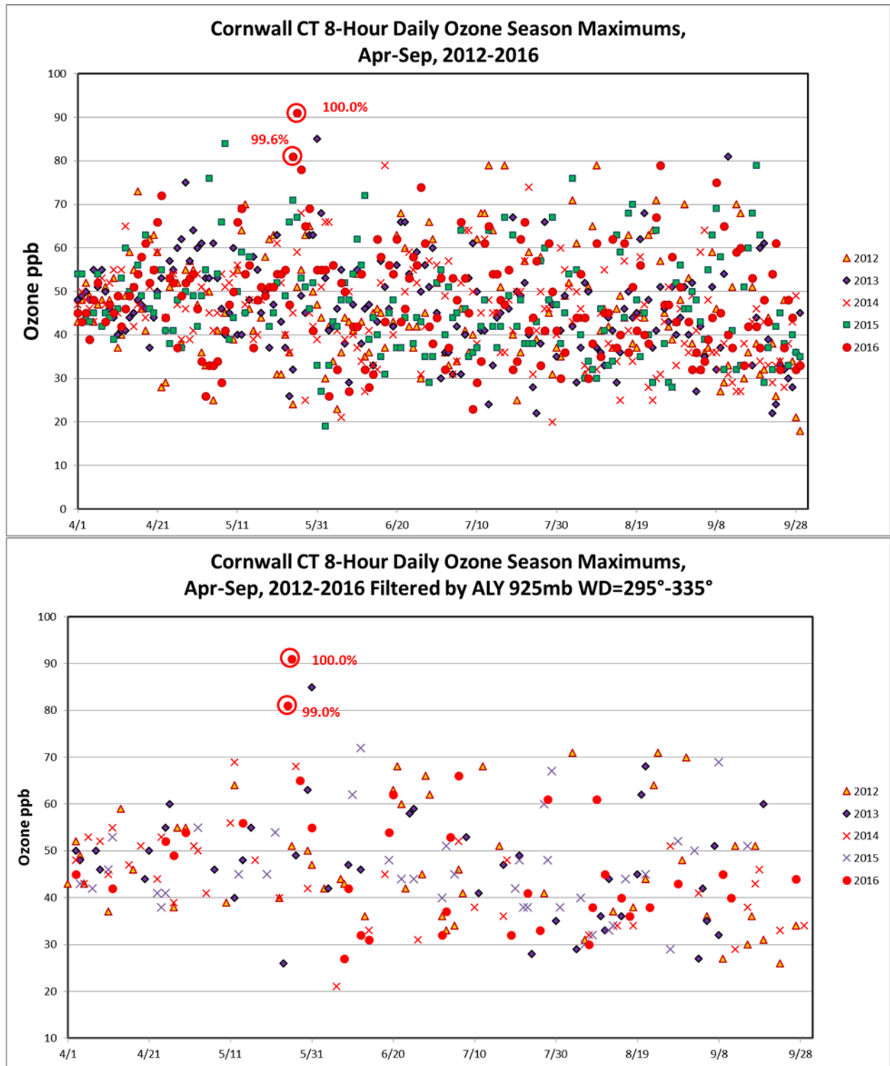
Figure 33. Cornwall CT Daily Ozone Season Maximums 2012-2016
