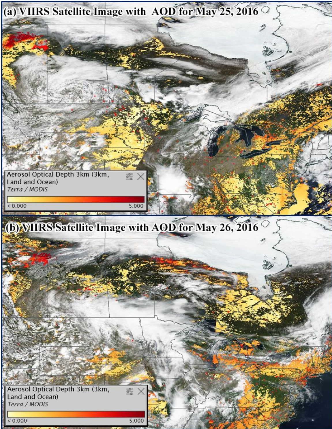
Figure 12. VIIRS Satellite Images. (a) May 25 th and (b) May 26 th , 2016 showing the Analyzed Aerosol Optical Depth (AOD) Associated with the Smoke Plume.
