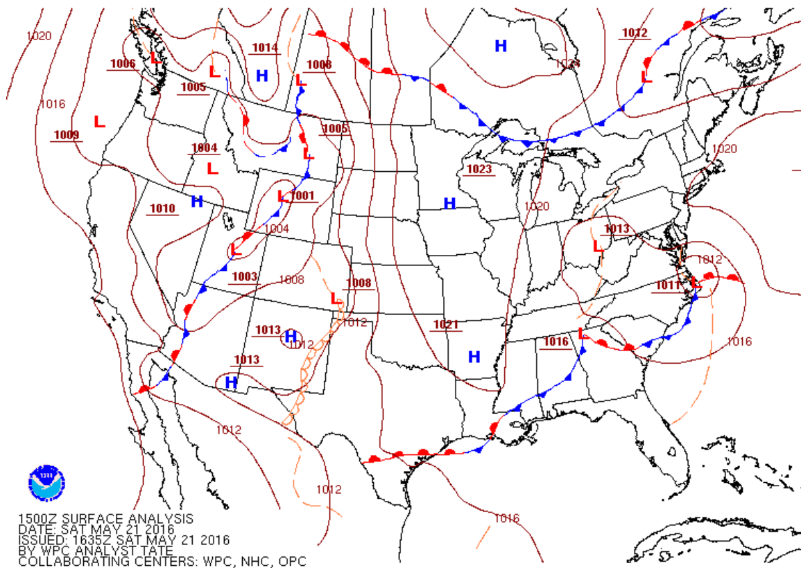
Figure 63. Surface Weather Analysis from May 21, 2016
