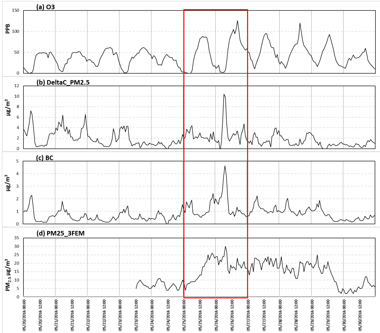
Figure 42. Monitored (a) Ozone, (b) DeltaC PM2.5, (c) Black Carbon (BC), and (d) PM2.5 at the Danbury CT Monitor
