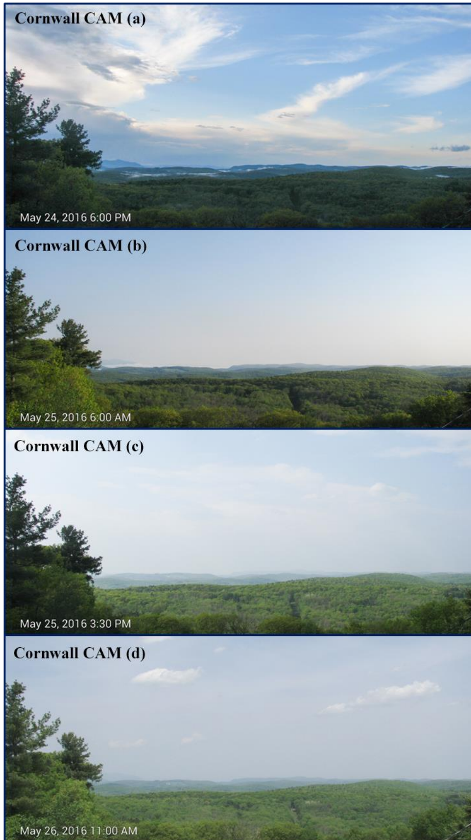
Figure 18. Cornwall Connecticut Webcam. (a)May 24-6:00pm, (b)May 25-6:00am), (c)May 25- 3:30pm and (d)May 26-11:00am, 2016.
