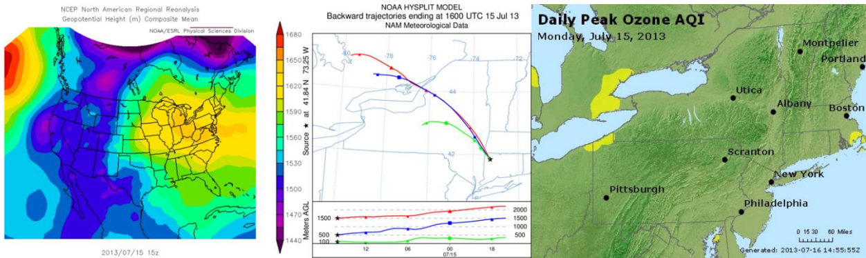
Figure 84. Matching 850 mb Pressure Pattern with Back Trajectories July 15, 2013.
