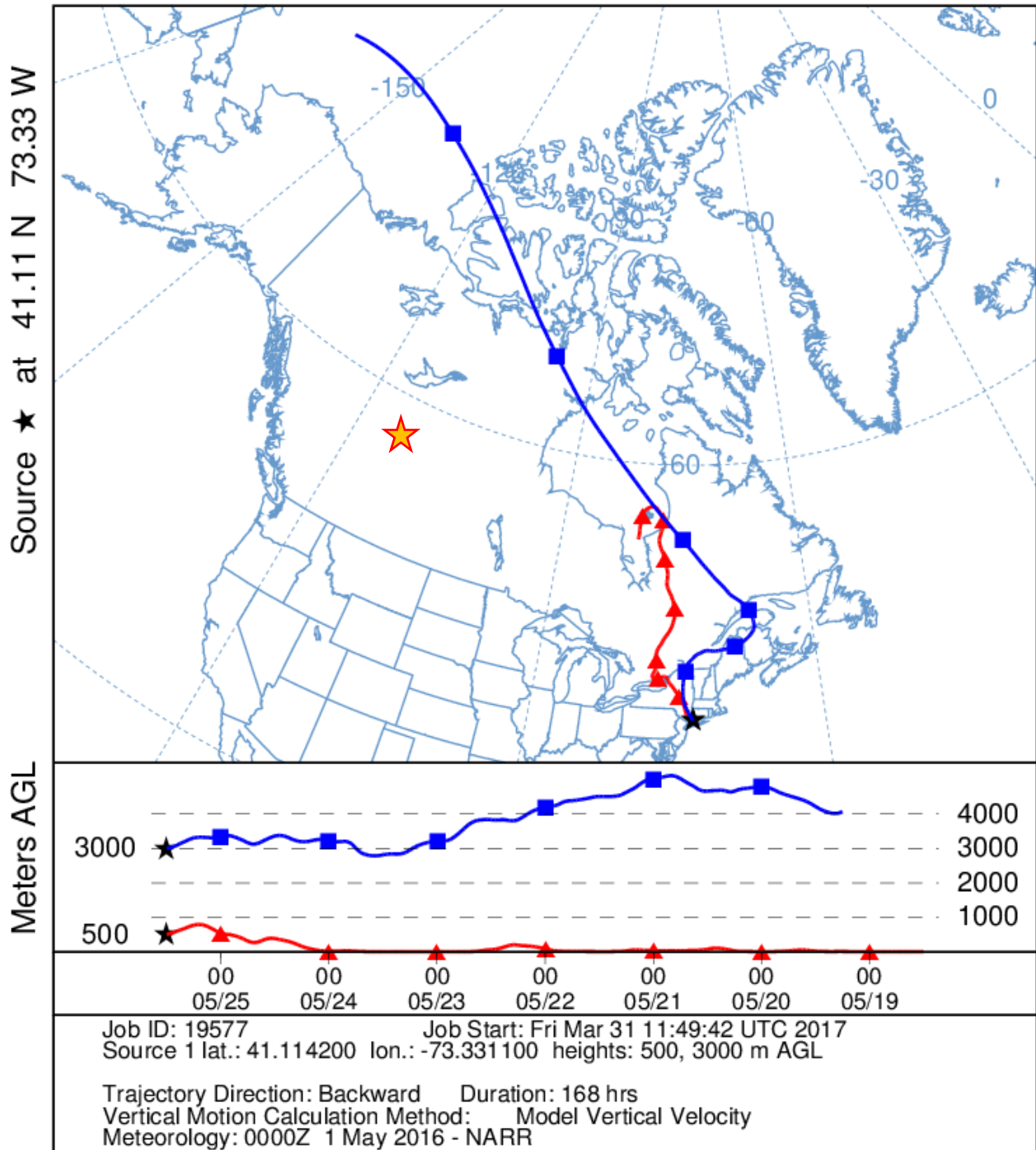
Figure 67. May 25, 2016 12 UTC Back Trajectories from Westport CT.
