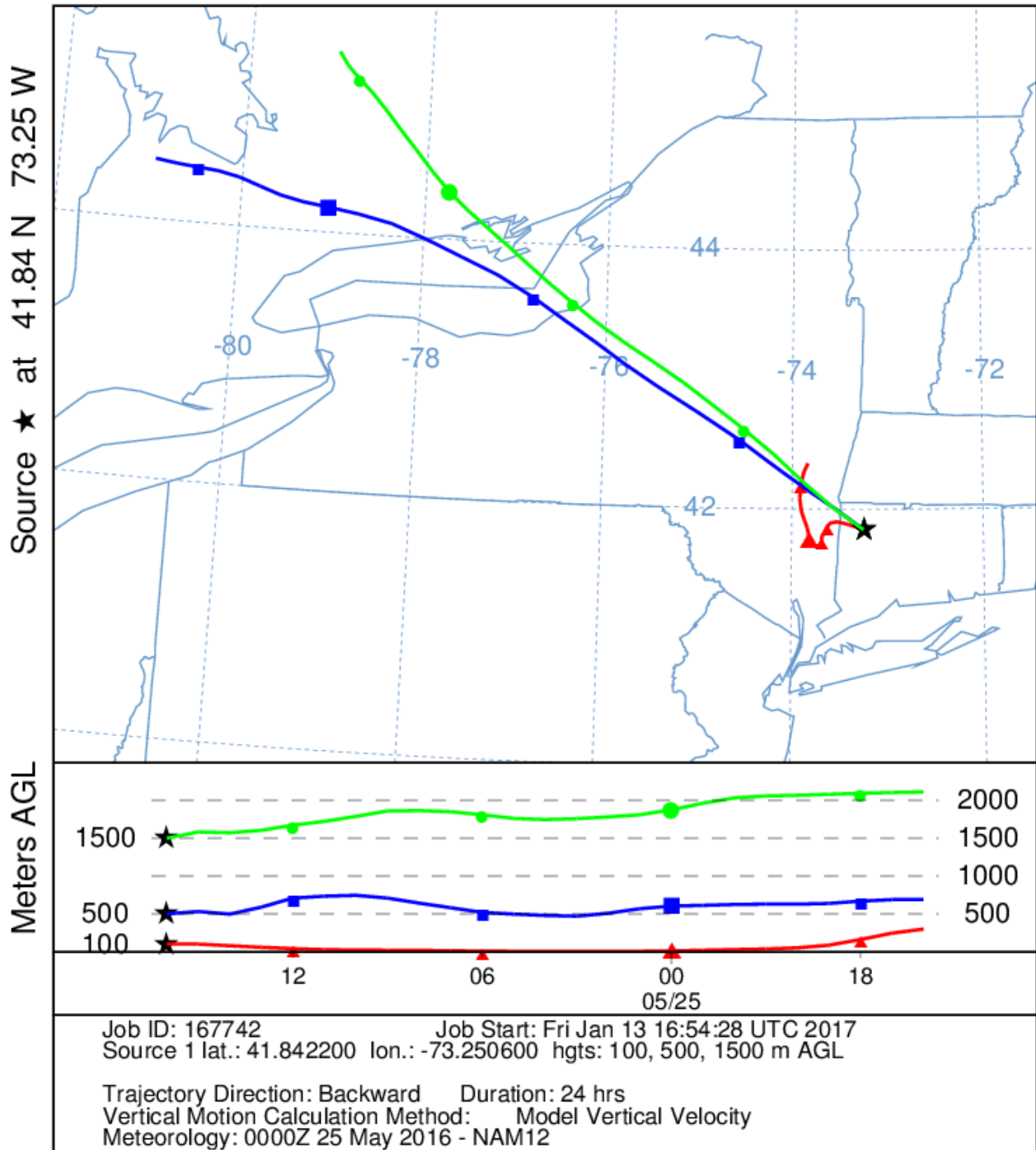
Figure 81. HYSPLIT Reference Trajectories from May 25th, 2016
