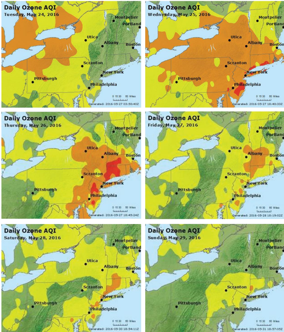
Figure 92. AQI Map of the Event.
