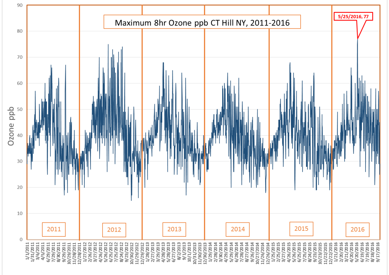
Figure 45. Monitored Daily Maximum 8-hour Ozone for 2011-2016 at Connecticut Hill, NY
