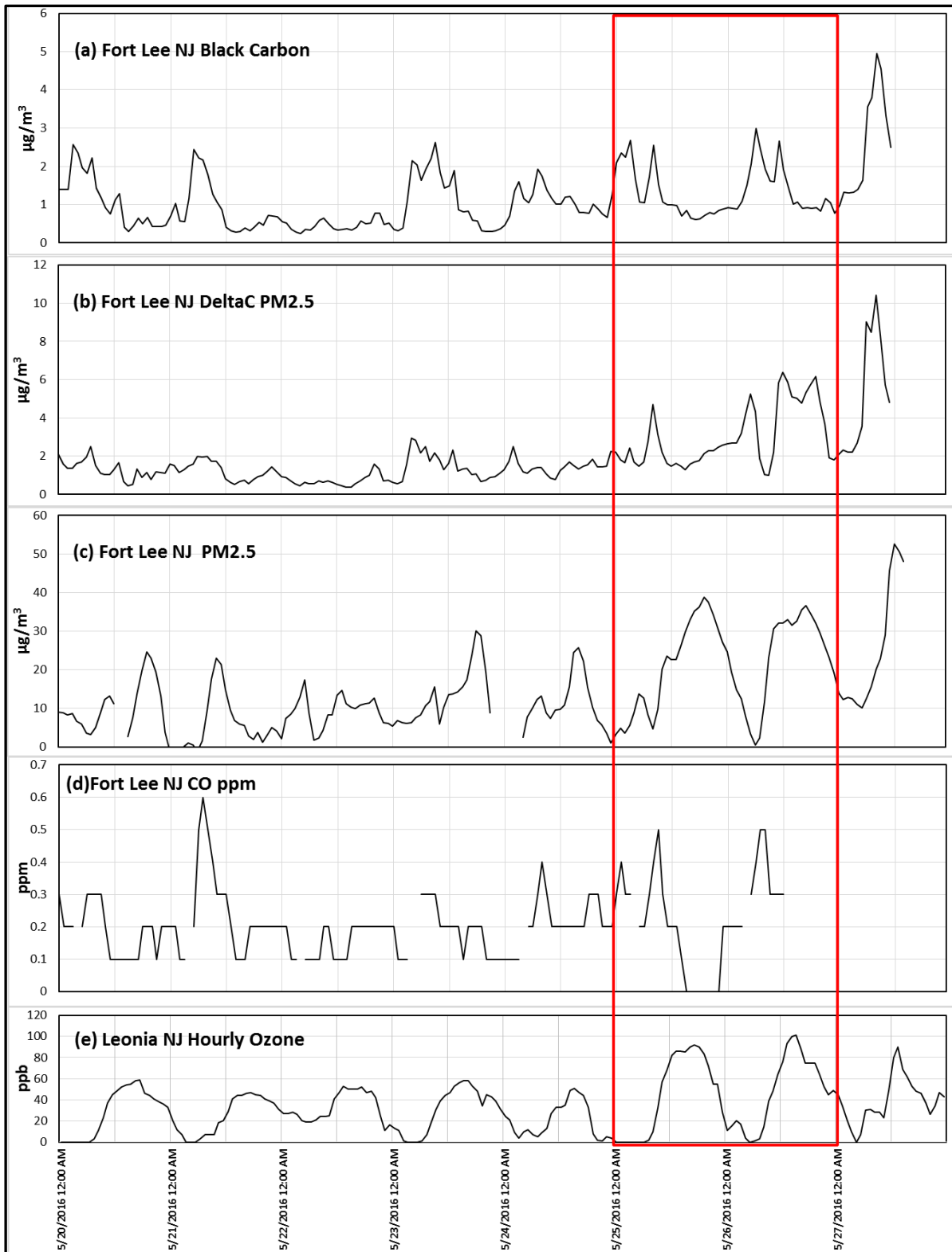
Figure 44. Monitored (a) Black Carbon, (b) DeltaC PM2.5, (c) PM2.5 (d) CO at the Fort Lee NJ monitor and (e) Ozone at the Leonia NJ Monitor.
