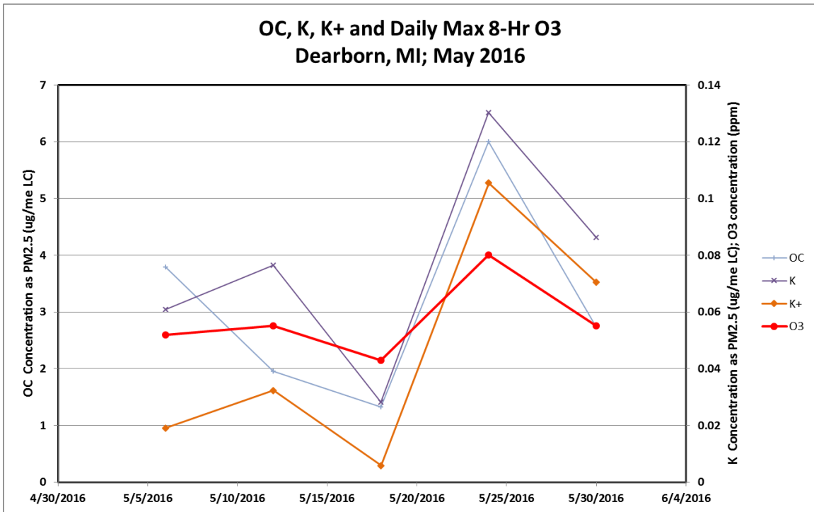
Figure 49. Dearborn Michigan CSN Data
