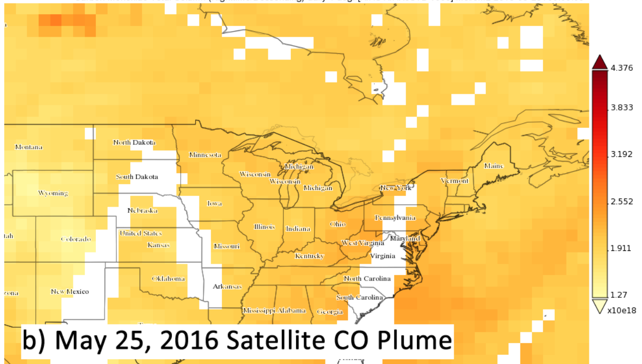
Figure 15. Satellite CO Plume from May 24 (a) and May 25 (b) , 2016. The elevated CO plume settles over the Midwest States and moves east into Connecticut.
