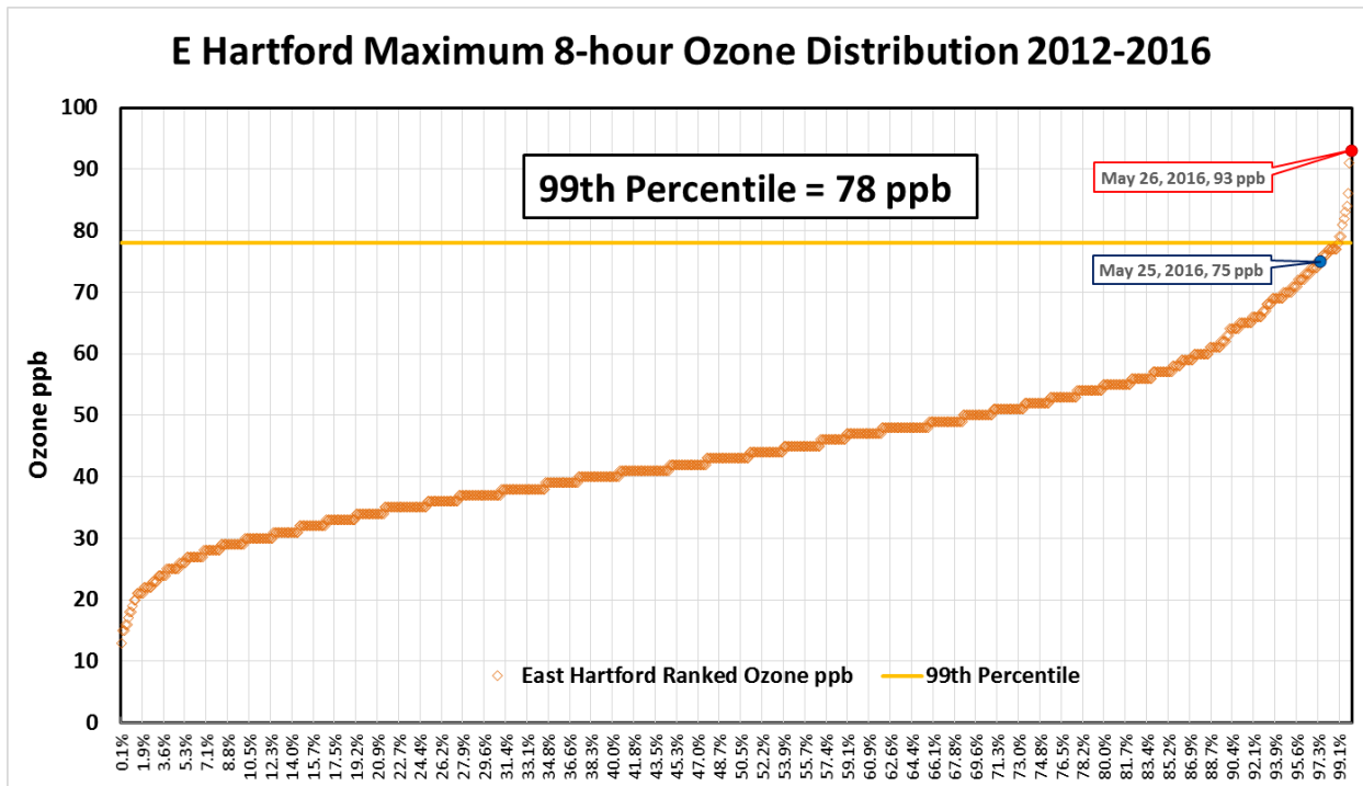
Figure 32. Ranked 8-hour Ozone Distribution for E Hartford CT 2012-2016
