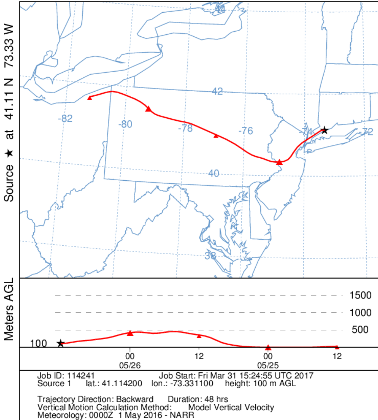
Figure 74. 100 meter Back Trajectory from Westport Connecticut ending at 8:00 am LDT, May 26, 2016.
