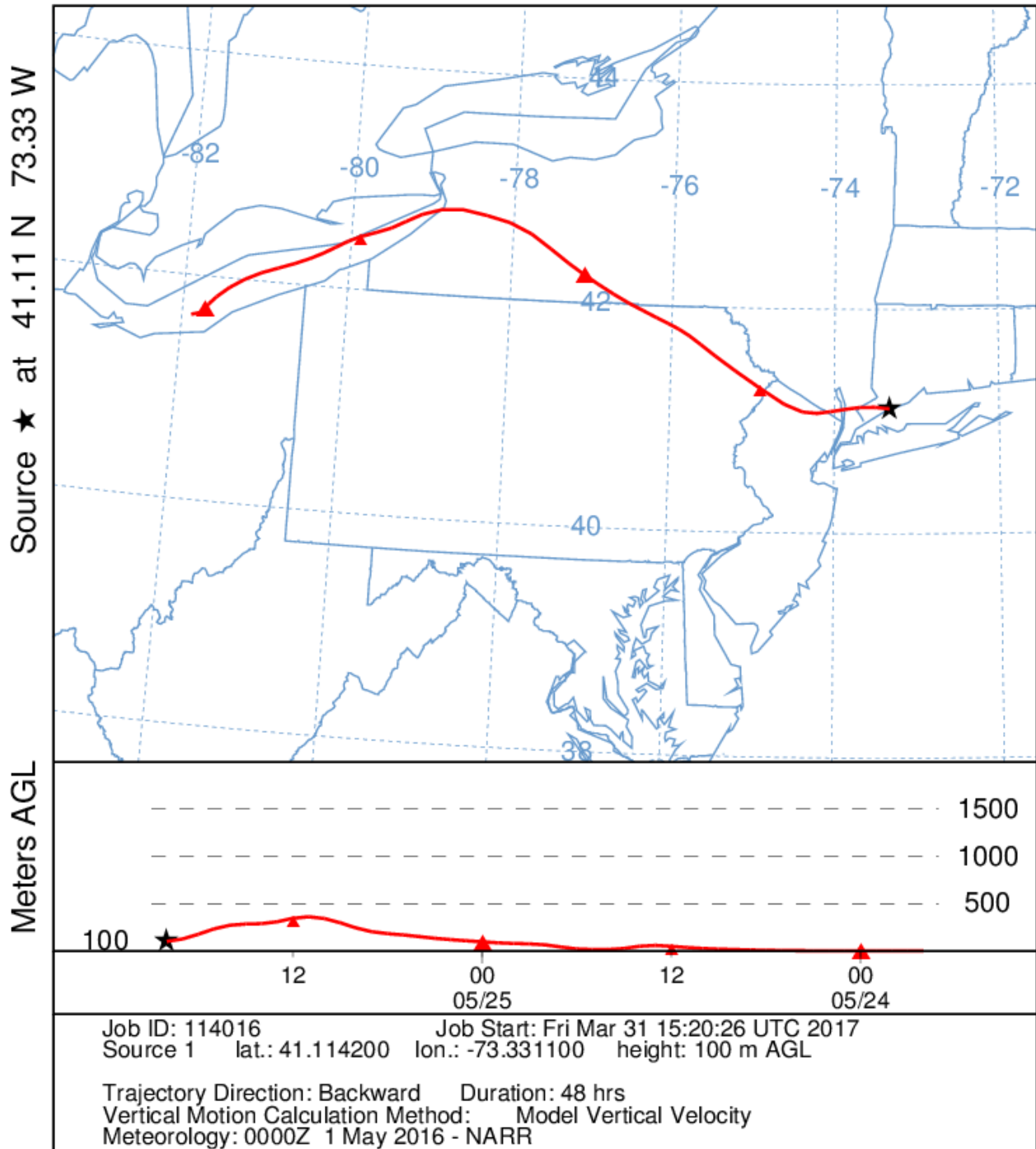
Figure 73. 100 meter Back Trajectory from Westport Connecticut ending at 4:00pm LDT, May 25, 2016.
