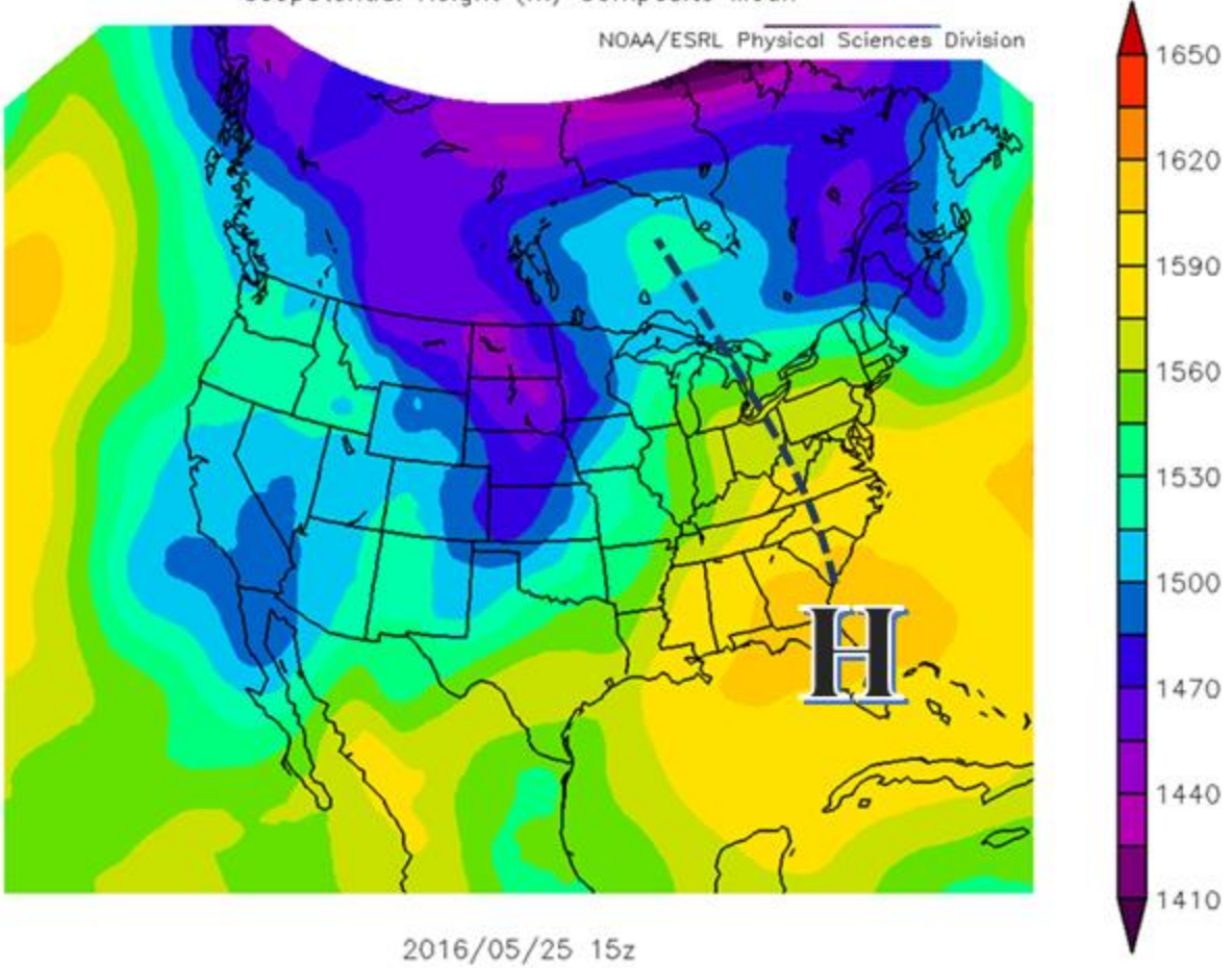
Figure 80. 850 mb Reference Pressure Pattern for May 25th, 2016
