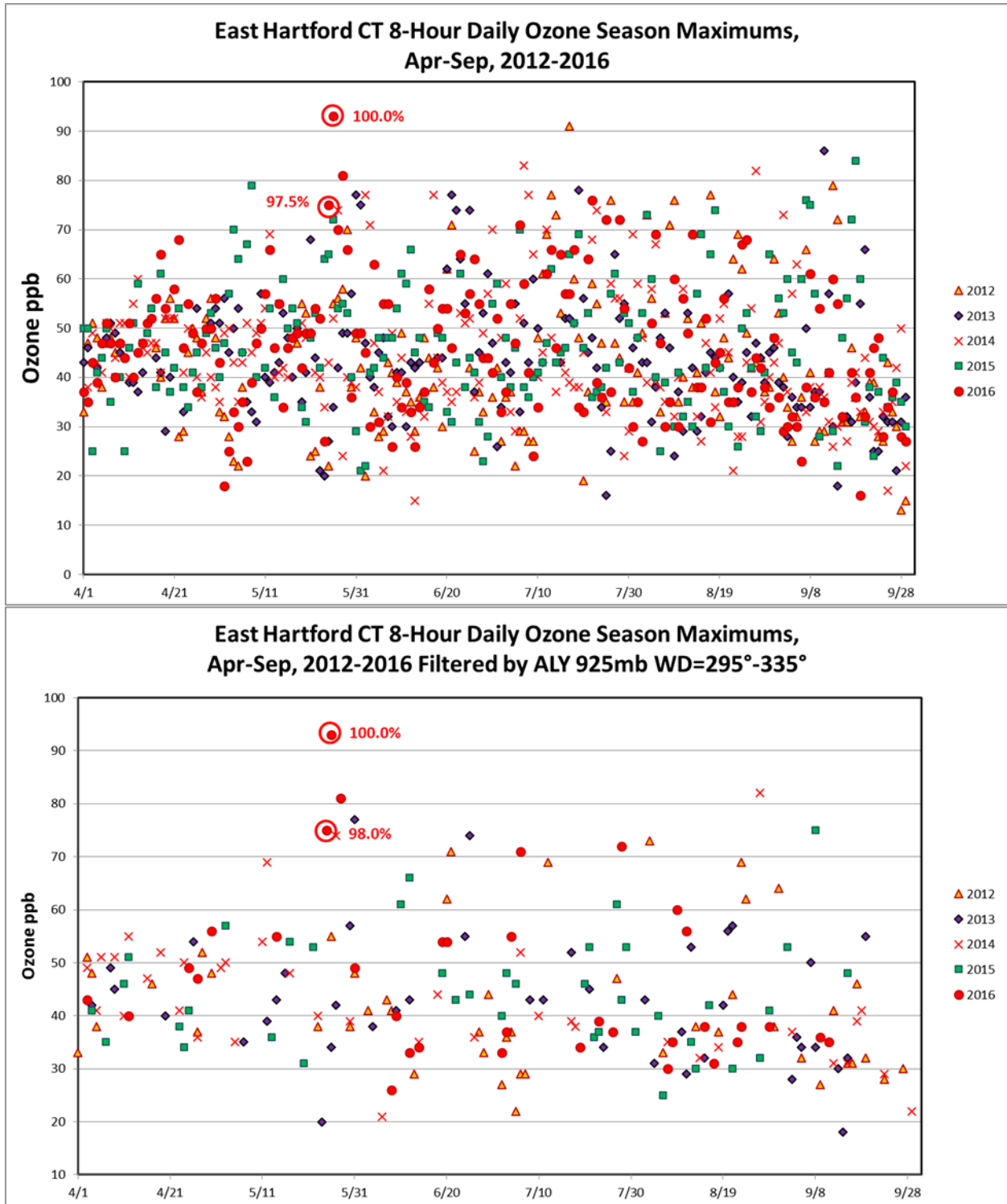
Figure 34. East Hartford CT Daily Ozone Season Maximums 2012-2016
