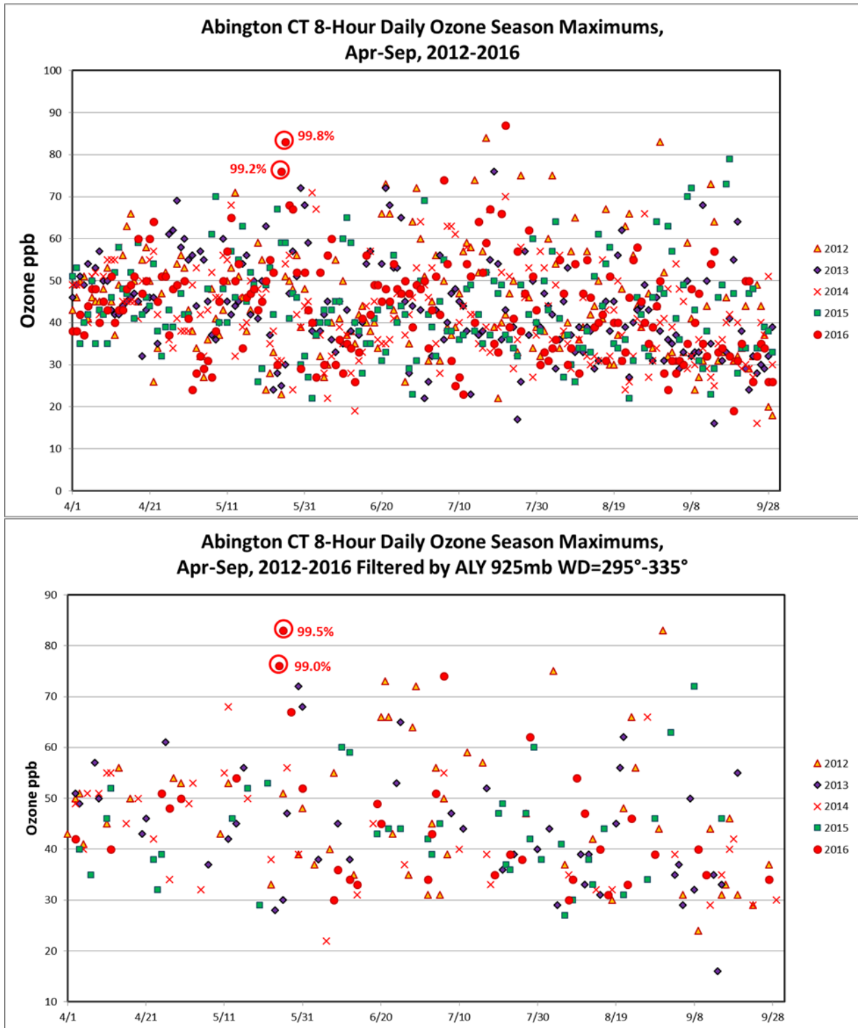
Figure 35. Abington CT Daily Ozone Season Maximums 2012-2016
