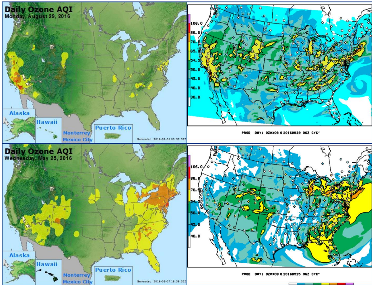
Figure 87. Comparing Similar Day Model Output from August 29th to May 25, 2016 with Observed AQI
