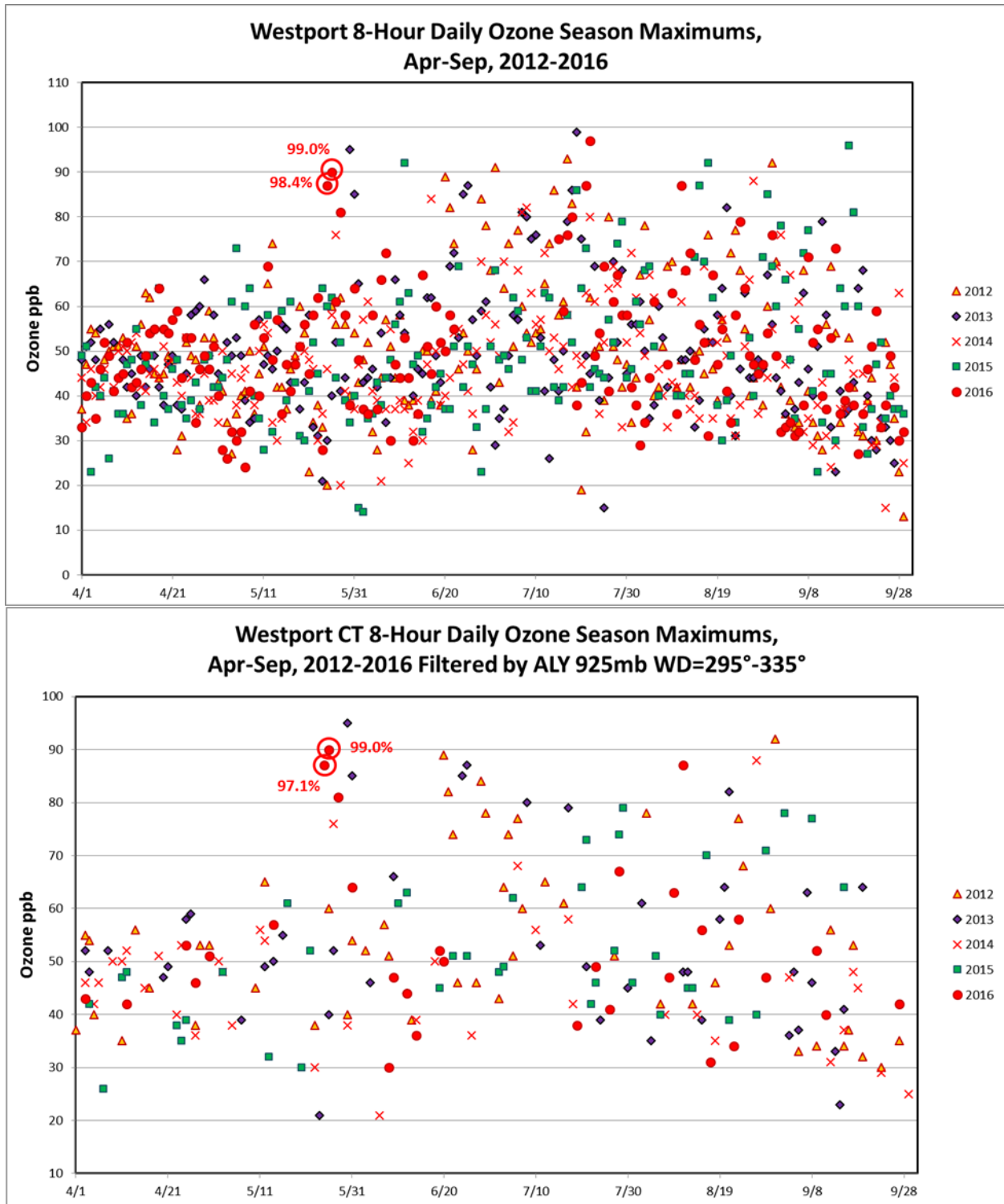
Figure 36. Westport CT Daily Ozone Season Maximums 2012-2016
