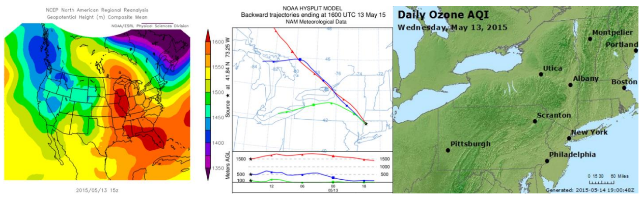
Figure 86. Matching 850 mb Pressure Pattern with Back Trajectories May 13, 2015
