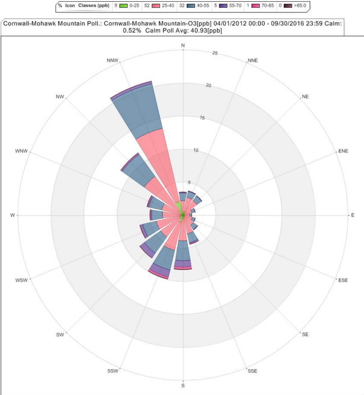
Figure 24. Ozone Wind Rose from Cornwall Connecticut.
