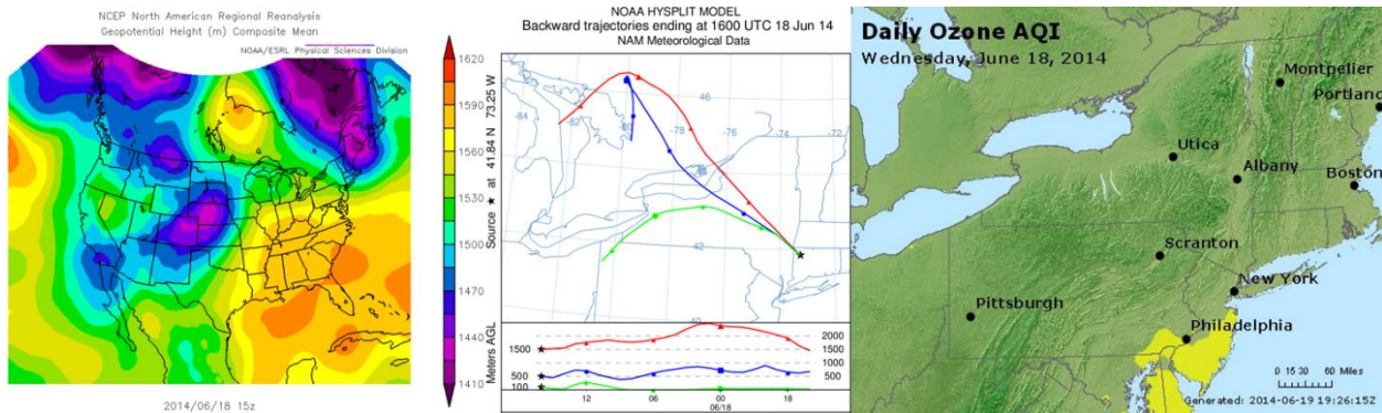
Figure 83. Matching 850 mb Pressure Pattern with Back Trajectories June 18, 2014.
