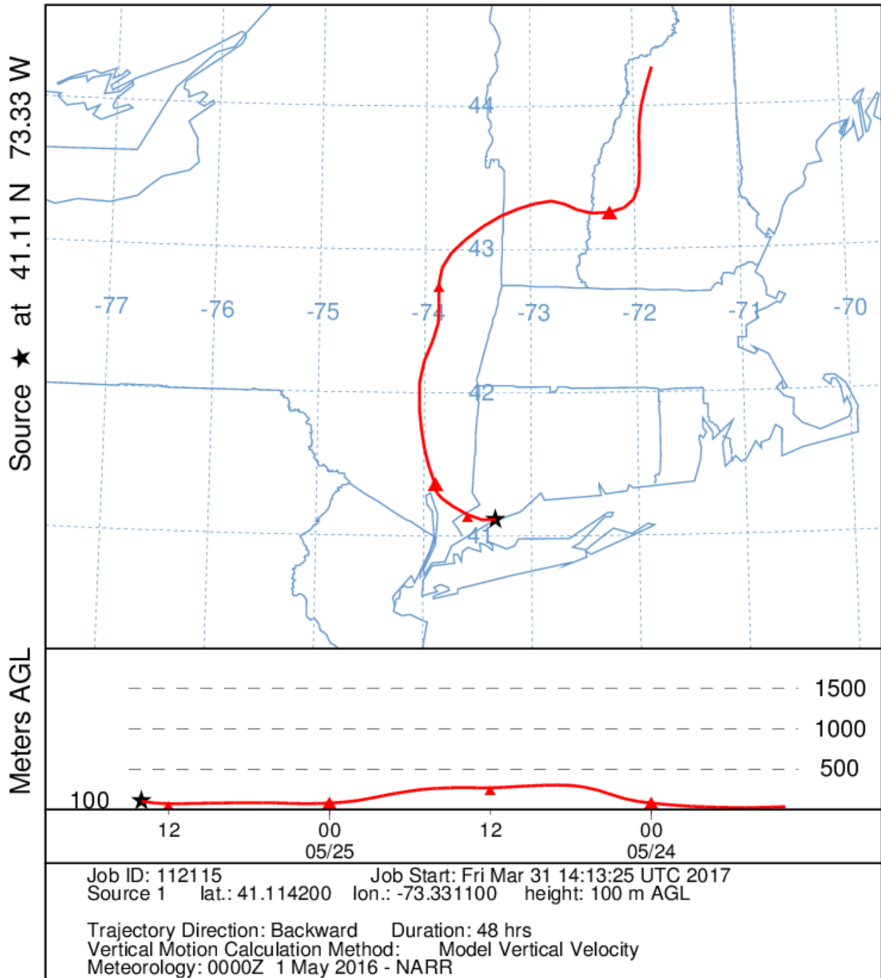
Figure 72. 100 meter Back Trajectory from Westport Connecticut ending at 10:00 am LDT May 25, 2016.
