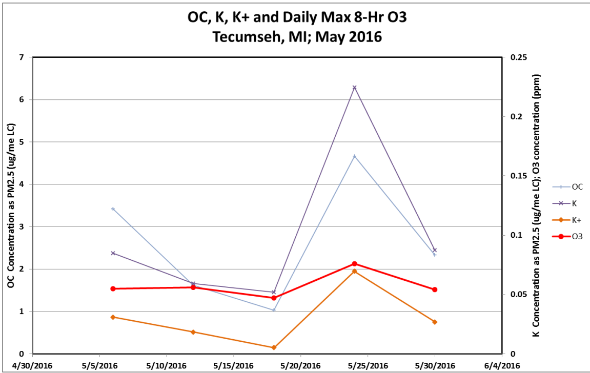
Figure 53. Tecumseh Michigan CSN Data
