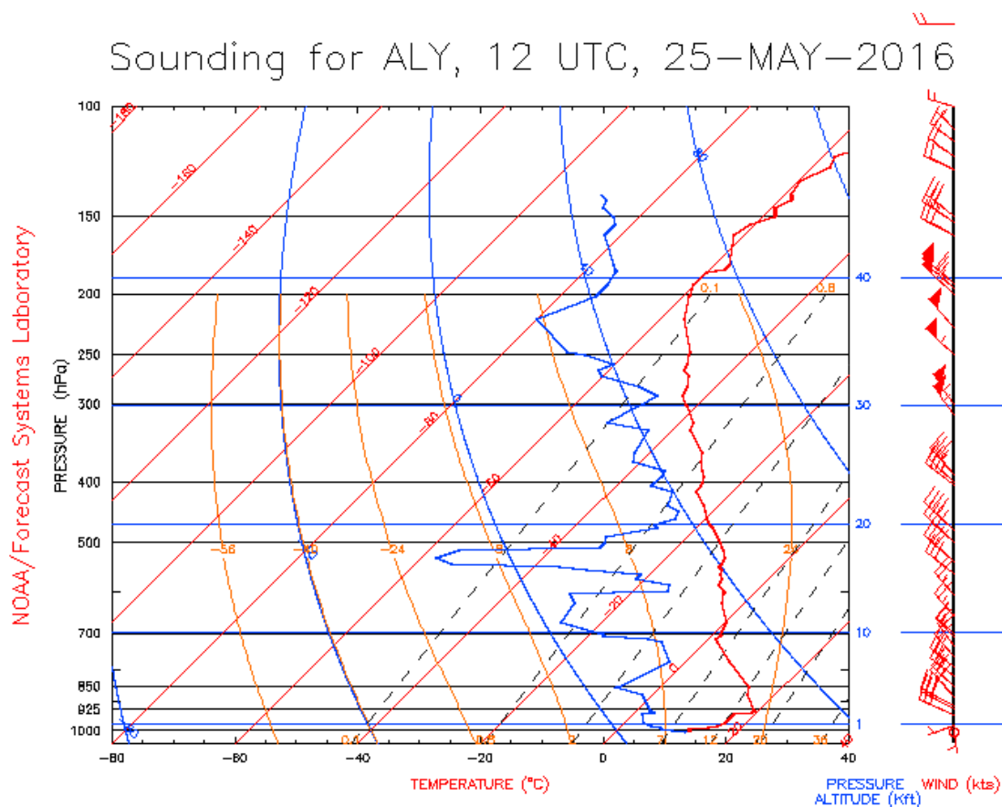
Figure 79. 12z ALY Sounding from May 25 th , 2016
