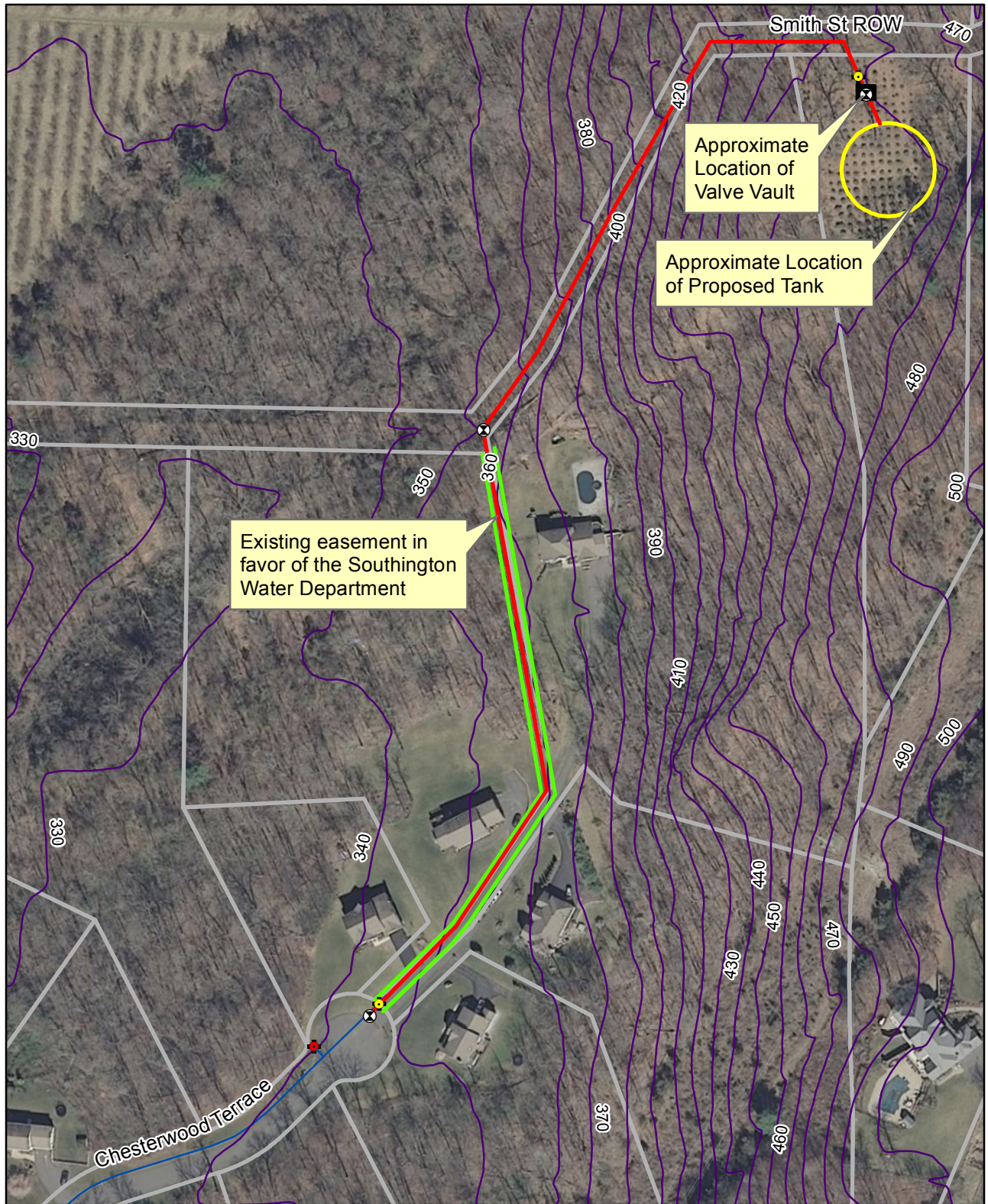
Figure 2 Proposed Water Storage Tank and Transmission Main Southington Water Department
