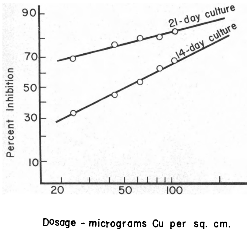
FIGURE 3. The influence of age of the culture used as a source of spores on the slope of the dosage-response curve. The fungicide is copper silicate and the fungus is Macrosporium sarcinaeforme .
